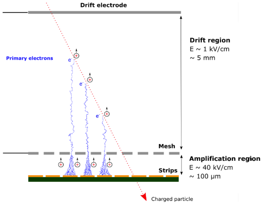
Figure 3.6: Micromegas detector.
