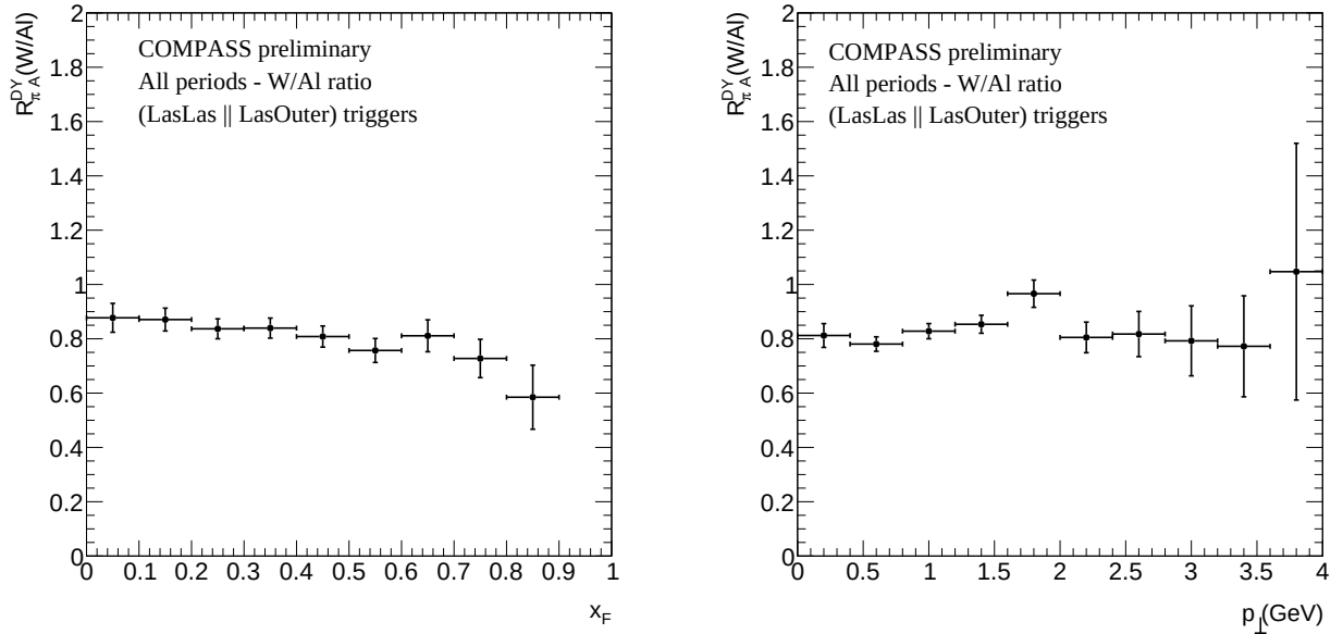
Figure 5.11: DY nuclear production ratio measured in \pi W normalised to \pi Al collisions as a function of x_F (left panel) and p_\perp (right panel) for all periods and the statistical error associated.
