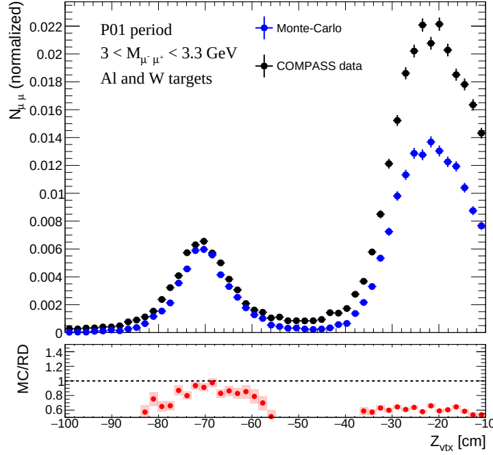
Figure 4.18: Comparison between the J/\psi MC (blue) and the P01 RD (black) for M \in (3 - 3.3) events normalised by the integral of the respective distributions as a function of Z_{\text{vtx}} .
