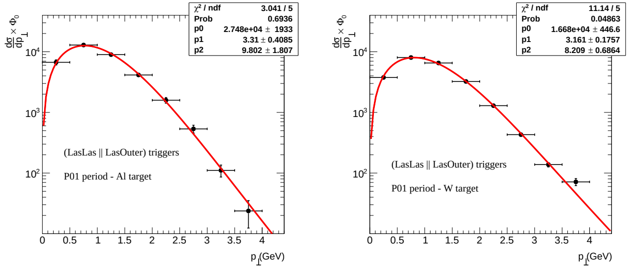
Figure 4.28: Kaplan fit of the absolute cross section as a function of p_\perp (GeV) multiplied by the initial absolute flux \Phi_0 for the Al (left panel) and the W (right panel) target in the P01. The error bars include statistical uncertainties only. The p_0 , p_1 and p_2 are respectively the parameters to the fit results corresponding to \mathcal{N} , p_0 and m in Eq. (7.8).
