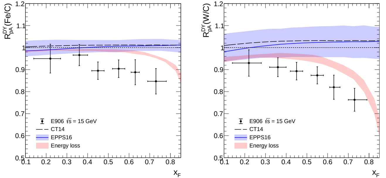
Figure 6.1: E906 nuclear production ratio measured in pFe (left panel) and pW (right panel) normalised to pC collisions at \sqrt{s} = 15 GeV compared to the EPPS16 nPDF calculation (blue band), isospin (dashed line) and energy loss effects (red band).
