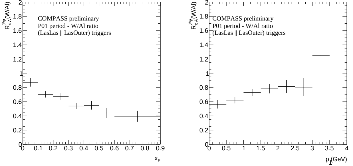
Figure 4.27: J/\psi nuclear production ratio measured in \pi W normalised to \pi Al collisions as a function of x_F (left panel) and p_\perp (right panel) for the period P01. The error bars include statistical uncertainties only.
