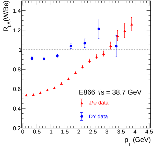
Figure 2.11: Ratio of DY (in blue) data ( 4 < M < 8.5 GeV) and J/\psi (in red) data ( 0.3 \leq x_F \leq 0.93 ) measured in pA collisions at \sqrt{s}=38.7 GeV as a function of the dimuon p_\perp from E866/NuSea experiment.
