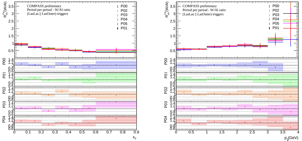
Figure 4.33: R_{\pi A}^{J/\psi}(\text{W}/\text{Al}) as a function of x_F (left panel) and p_\perp (right panel) from the different periods (P00, P01, P02, P03 and P04) and the statistical uncertainties associated (top). The ratio between R_{\pi A}^{J/\psi}(\text{W}/\text{Al}) as a function of x_F (left panel) and p_\perp (right panel) from different periods (P00, P01, P02, P03 and P04) normalized by the period P01.
