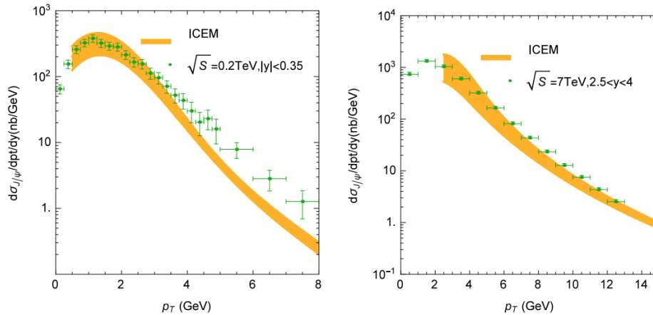
Figure 1.12: Comparison between ICEM model [51] (in orange) and data as a function of p_\perp from prompt J/\psi production in pp collisions at \sqrt{s} = 200 \text{ GeV} and \sqrt{s} = 7 \text{ TeV} from RHIC experiment at mid rapidity [66] and from LHCb experiment at forward rapidity [67] respectively.
