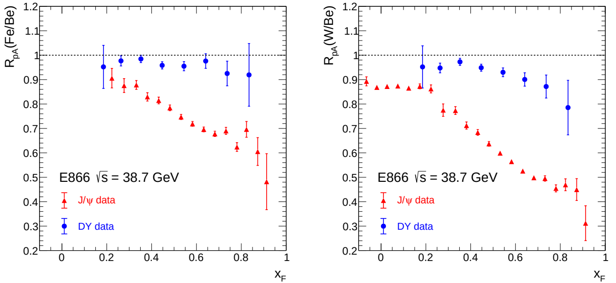
Figure 2.10: Ratio of DY (in blue) ( 4 < M < 8.5 GeV) and J/\psi (in red) data measured in pA collisions at \sqrt{s}=38.7 GeV as a function of the x_F from E866/NuSea experiment in Fe (left panel) and W (right panel) nucleus, both normalised to the Be target.
