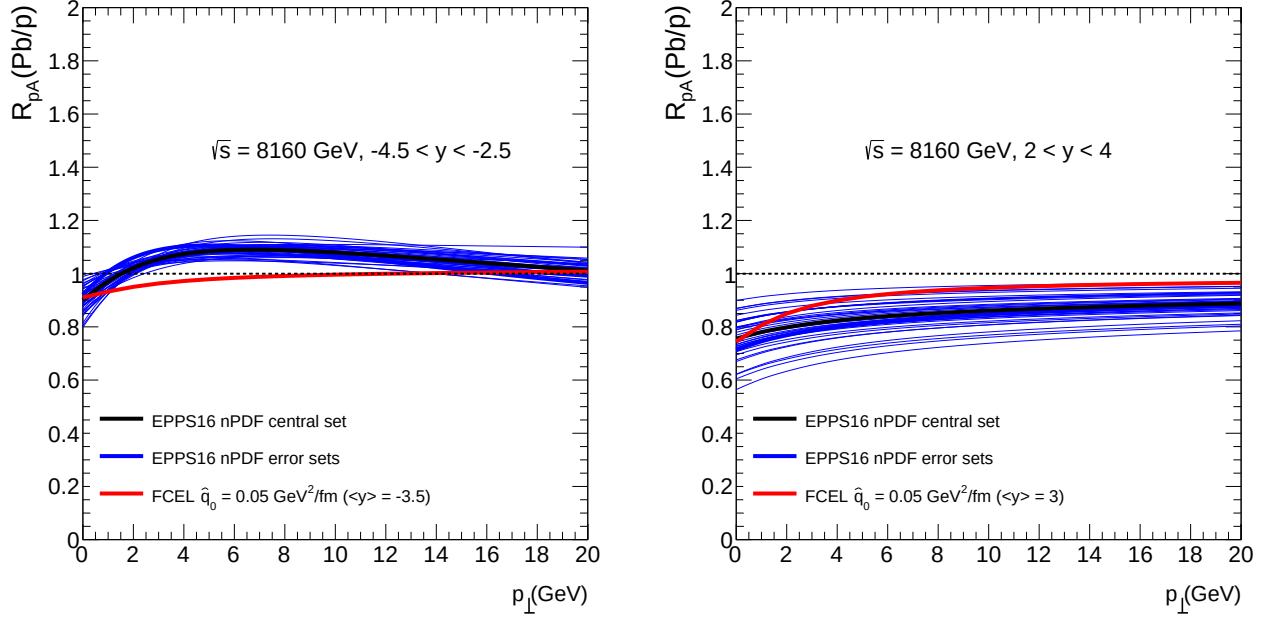
Figure 7.5: R_{pA}^{J/\psi} (Pb/p) as a function of p_{\perp} calculated with the EPPS16 nPDF and FCEL effects at \sqrt{s} = 8160 GeV in backward, -4.5 < y < -2.5 , (left panel) and forward, 2 < y < 4 (right panel) rapidity.
