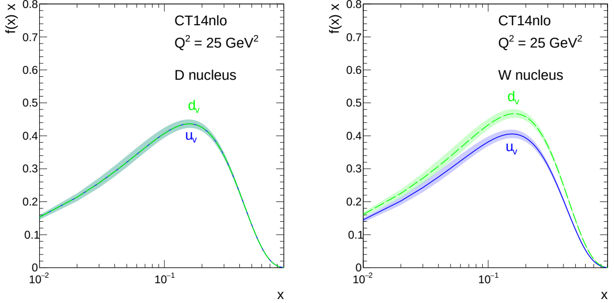
Figure 2.1: Parton distribution functions of u_v^A(x) and d_v^A(x) normalised by A times x and their associated uncertainties at Q^2 = 25 \text{ GeV}^2 for deuterium nucleus (left panel) and tungsten nucleus (right panel) at Next-to-Leading Order (NLO) using CT14 parameterization [28].
