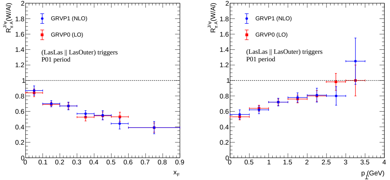
Figure 4.32: Impact of the pion PDF used in J/\psi MC simulation on the R_{\pi A}^{J/\psi}(W/Al) ratio as a function of x_F (left panel) and p_\perp (right panel). In blue, R_{\pi A}^{J/\psi}(W/Al) ratio using an acceptance calculation using GRVP1 (NLO) and in red, using an acceptance calculation using GRVP0 (LO) [34].
