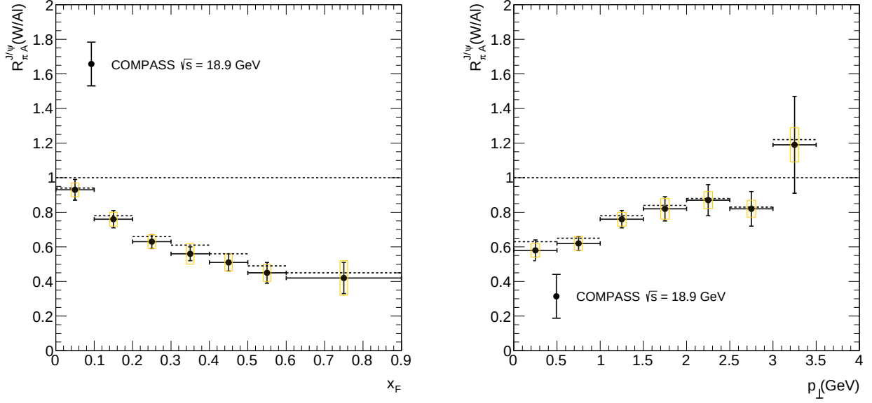
Figure 4.35: R_{\pi A}^{J/\psi}(W/Al) mean values as a function of x_F (left panel) and p_\perp (right panel) from nine periods. The black errors bars and the yellow squares represent the statistical and systematic uncertainties, respectively. The black dotted line corresponds to the low limit due to the underestimation of the contamination of the J/\psi events due to the migration from the W to the Al target.
