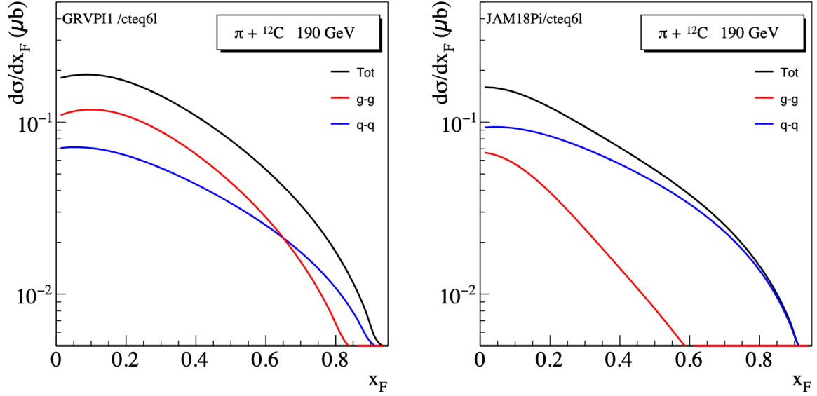
Figure 2.3: Differential J/\psi cross section using the CEM model at LO at E_{\text{beam}}=190 GeV in \pi^-A collisions using the GRV (left panel) and JAM pion PDFs (right panel).
