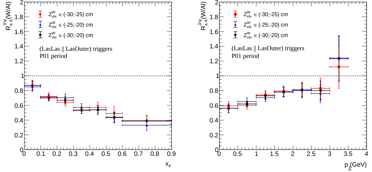
Figure 4.31: Impact of the Z_{\text{vtx}} cut in the W target on the R_{\pi A}^{J/\psi}(W/Al) ratio as a function of x_F and p_\perp . In blue, J/\psi extracted by fitting the dimuon invariant mass in second 5 cm in the W target. In red, J/\psi extracted by fitting the dimuon invariant in first 5 cm in the W target and in black, the first 10 cm.
