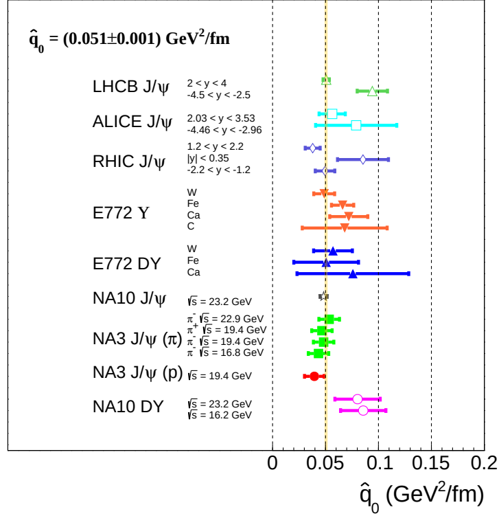
Figure 7.3: Extracted values of \hat{q}_0 from each measurement of \Delta p_\perp^2 . Experiments are plotted in descending order of \sqrt{s} energy, data points in ascending order of atomic number (E772) and rapidity (PHENIX, ALICE, LHCb).
