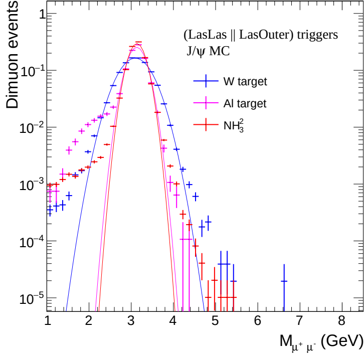
Figure 4.5: J/\psi MC distribution in the W (in blue), Al (in magenta) and \text{NH}_3^2 (in red) targets.
