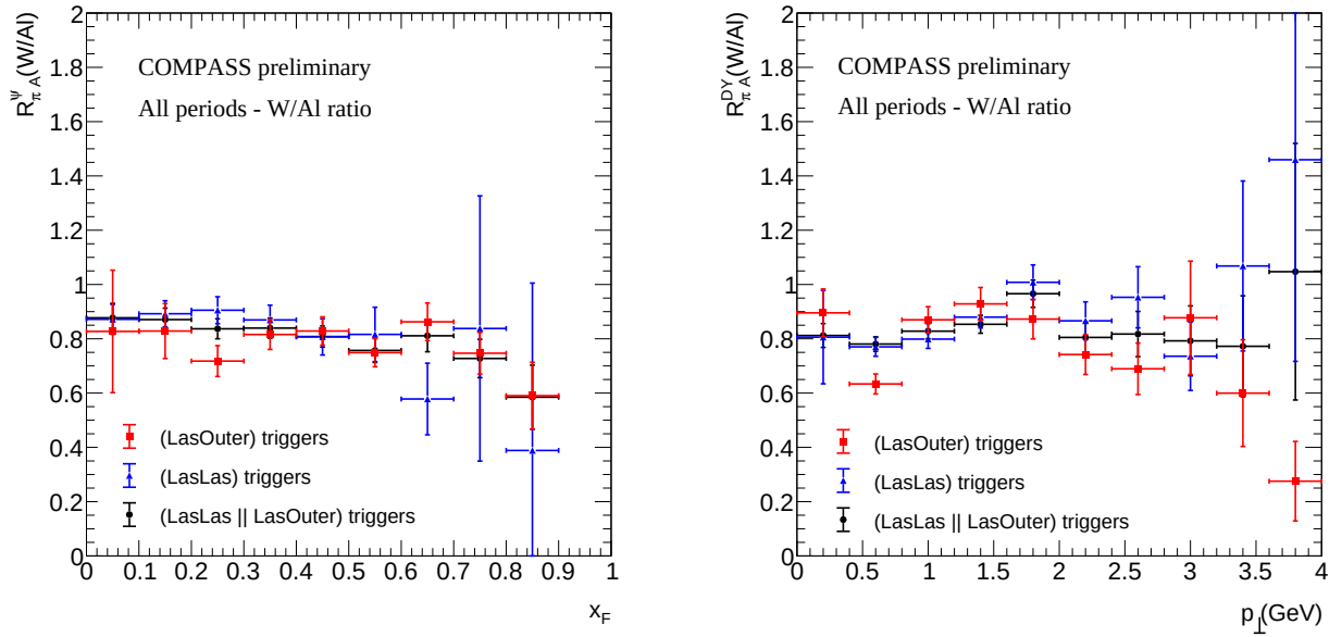
Figure 5.13: Impact of the triggers used in the R_{\pi A}^{\text{DY}}(\text{W/Al}) ratio as a function of x_F and p_\perp . In blue, R_{\pi A}^{\text{DY}}(\text{W/Al}) ratio calculated in LasLas trigger and in red, calculated in LasOuter trigger and in black, for both LasLas or LasOuter trigger.
