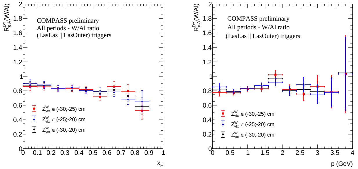
Figure 5.14: Impact of the Z_{\text{vtx}} cut of the W target on the R_{\pi A}^{\text{DY}}(\text{W/Al}) ratio as a function of x_F and p_{\perp} . In blue, R_{\pi A}^{\text{DY}}(\text{W/Al}) ratio calculated in second 5 cm in W target, in red, calculated in first 5 cm in W target and in black, in the first 10 cm.
