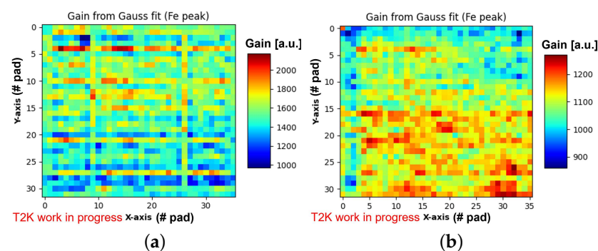
Figure 3. Map of gain for each pad of ERAM 11 (a) and ERAM 23 (b) obtained with X-ray test bench. Unexpected regular patterns are visible on ERAM 11.
