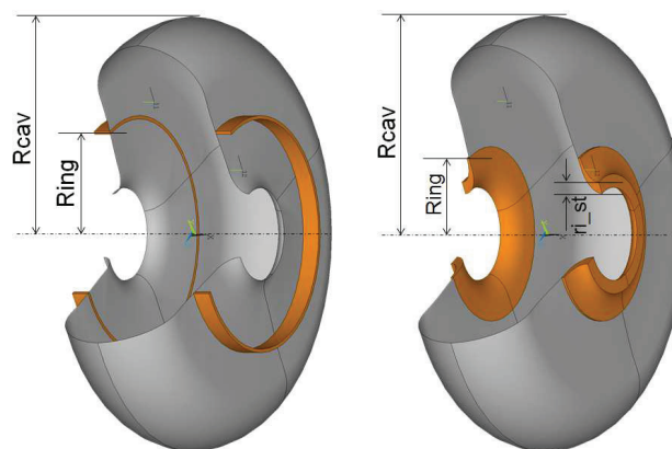
Figure 1: Elliptical mid-cell geometry ( \beta=0.61 ) with ring and iris stiffening options.
