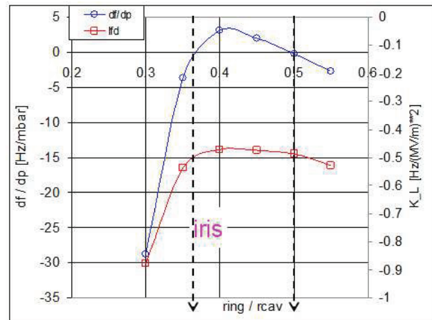
Figure 5: FNAL elliptical mid-cell ( \beta = 0.61 ) iris stiffening optimization.
