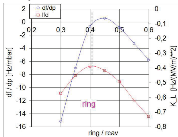
Figure 10: FNAL elliptical 5-cell cavity ( \beta=0.92 ) stiffening optimization with ring.
