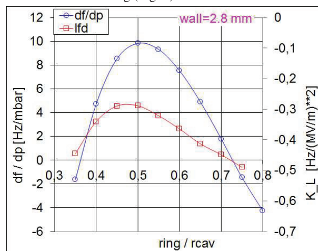
Figure 2: TeSLA mid-cell mechanical properties.
