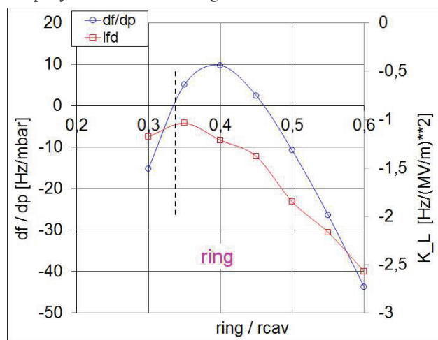
Figure 9: FNAL elliptical 5-cell cavity ( \beta=0.61 ) stiffening optimization with ring.
