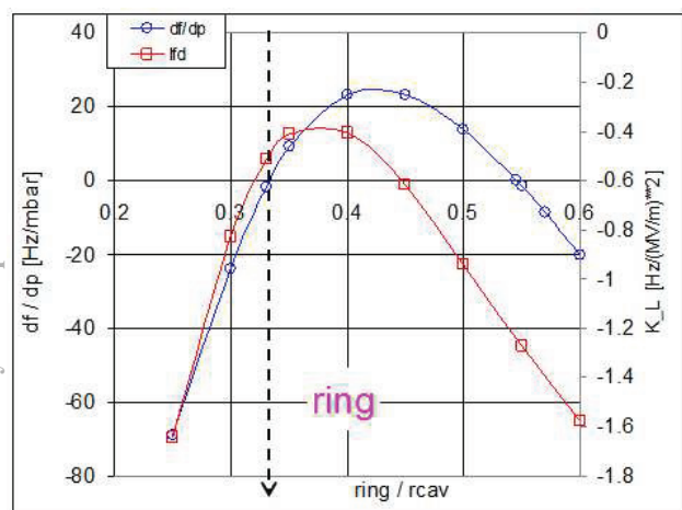
Figure 4: FNAL elliptical mid-cell ( \beta = 0.61 ) stiffening optimization with ring.
