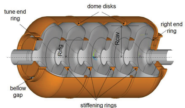
Figure 6: FNAL 5-cell elliptical cavity ( \beta = 0.61 ) simulation model with provisional helium vessel.
