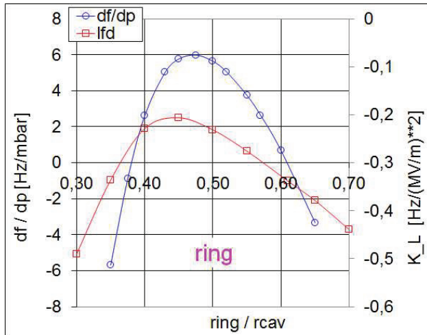
Figure 3: FNAL elliptical mid-cell ( \beta = 0.92 ) stiffening optimization with ring.
