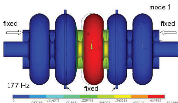
Figure 8: 1 st mechanical eigenmode of FNAL 5-cell elliptical cavity ( \beta=0.61 ) with dome disks.
