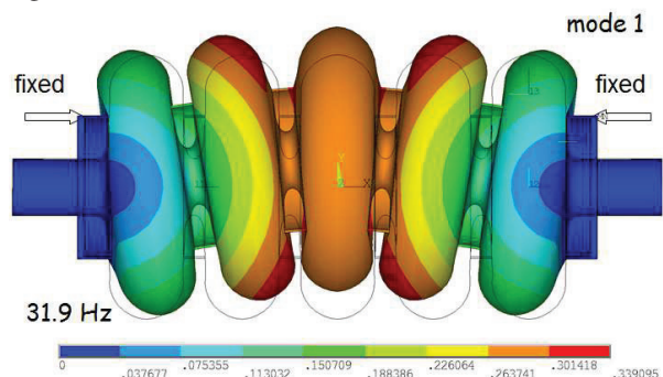
Figure 7: 1 st mechanical eigenmode of FNAL 5-cell elliptical cavity ( \beta=0.61 ).
