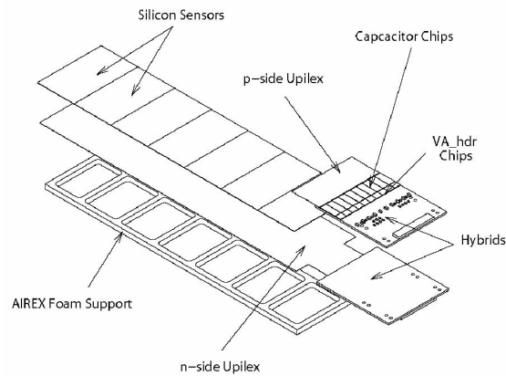
Figure 4: The principal components of the silicon ladder.
