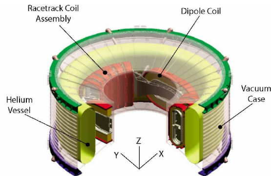
Figure 2: AMS-02 superconducting magnet layout.
