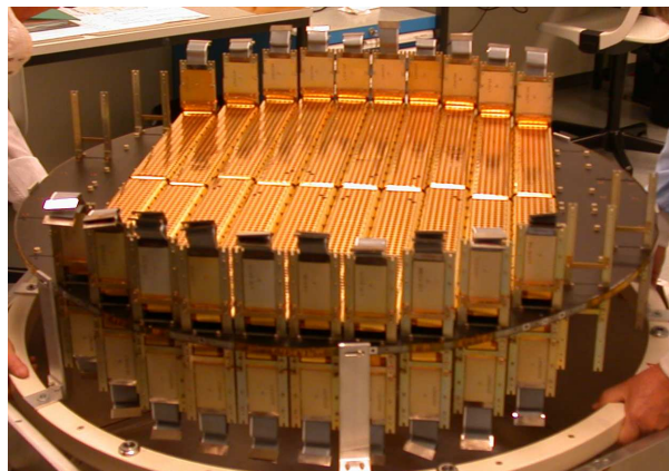
Figure 5: Plane numbers 2 completely equipped with ladders.
