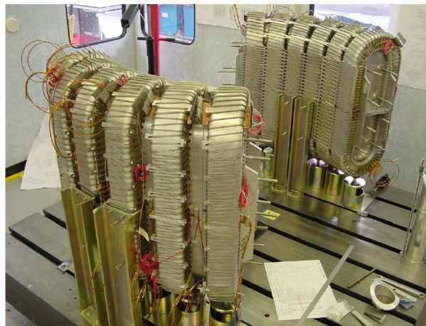
Figure 3: Coil Assembly.
