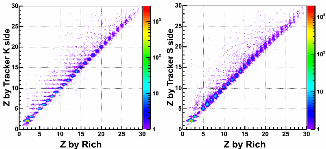
Figure 6: Comparisons of charge (Z) measurements by the Tracker and RICH.
