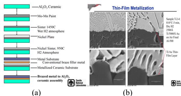
Figure 3: (a) The standard Mo-Mn process and (b) A thin film process using Ti and Au on AL500 Alumina achieving 12-14 ksi peel strength [7].
