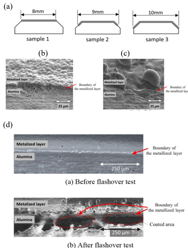
Figure 1: (a) Examples of the metalizing around a chamfer [1] (b) before processing, (c) changes to the triple junction region after high voltage processing [1], (d) Fig. 10 from Ref. [1], identifying the coated area which “eliminated” the triple junction region.
