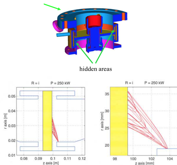
Figure 4: Coaxial choke design used at SNS [8].
