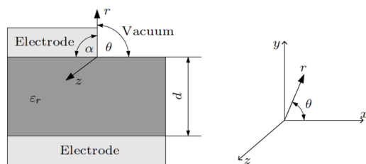
Figure 5: Modeling the triple junction with dielectric constant of the ceramic and angle of the electrode [9].
