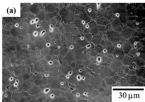
Figure 2: This example of alumina ( \text{Al}_2\text{O}_3 ) porosity is Fig. 1.4a from Ref. [6].
