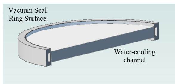
Figure 6: Conceptual elements of the mechanical design with a compression ring.
