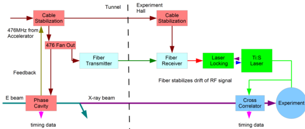
Figure 8: Timing Subsystems
