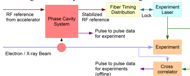
Figure 1: System Overview
