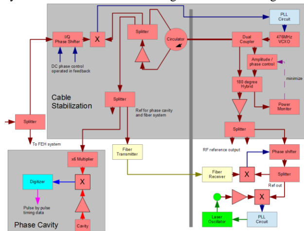
Figure 9: RF subsystem
