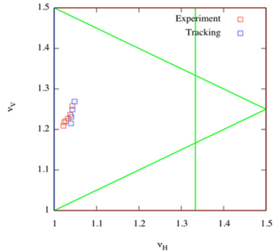
Figure 6: Betatron tunes. The red open squares show the betatron tunes obtained from the measurement and the blue ones from the beam tracking one, respectively.
