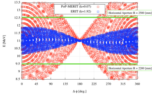
Figure 2: The longitudinal beam motions of fixed RF frequency acceleration for two different field indexes. The blue and red points show the beam motions for two different cases; one is for the field index of k = 1.92 and the other for k = 0.07 , respectively.
