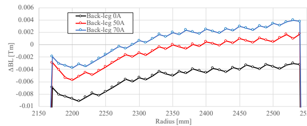
Figure 3: Magnetic field error at the RF cavity section. The vertical axis shows the field errors estimated from the difference of BL integrations with and without RF cavity.
