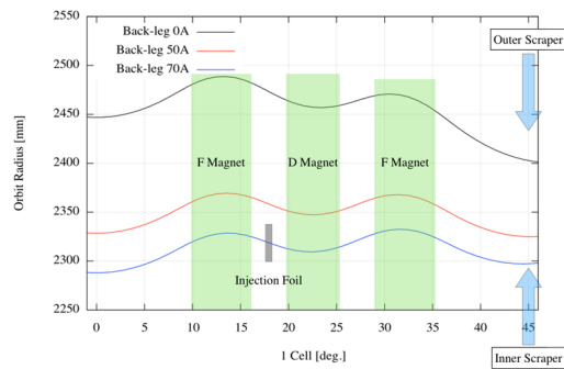
Figure 4: Closed orbit profiles for various back-leg coil currents at the injection point. The positions of the charge-exchange injection foil and scrapers are also shown in the figure.
