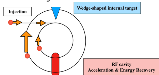
Figure 1: Schematic diagram of MERIT scheme.
