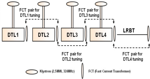
Figure 2: Phase Scan Signature Matching Technique using FCT pairs
