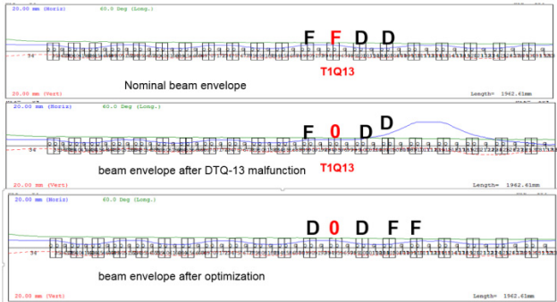
Figure 4: Beam envelope simulation results.
