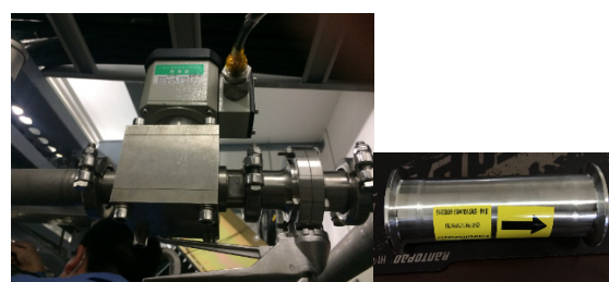
Figure 8: Flow meter and straight pipe.
