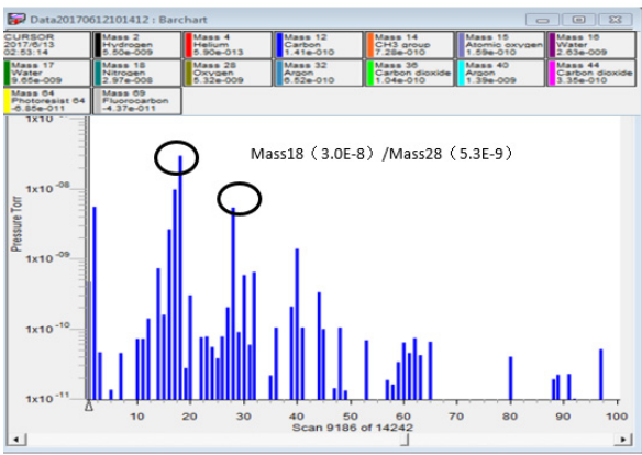
Figure 3: Residual gas spectrum in DTL1.
