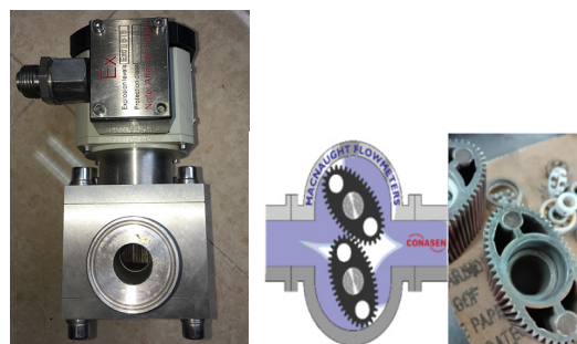
Figure 7: Schematic of flow meter.
