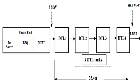
Figure 1: Layout of the CSNS LINAC.
