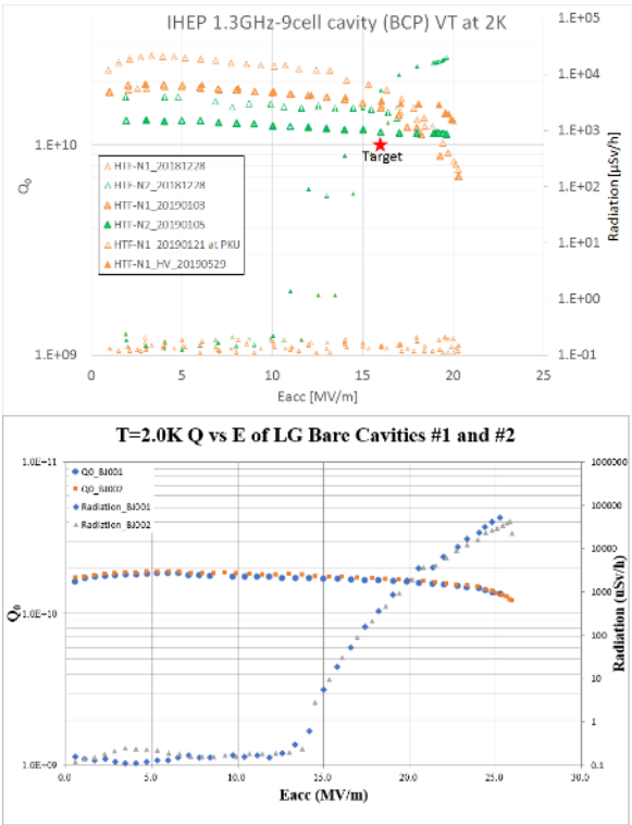
Figure 3: vertical testing results of SHINE 1.3 GHz prototype cavities at 2K. Up: FG cavities by Group-1. Bottom: LG cavities by Group-2.
