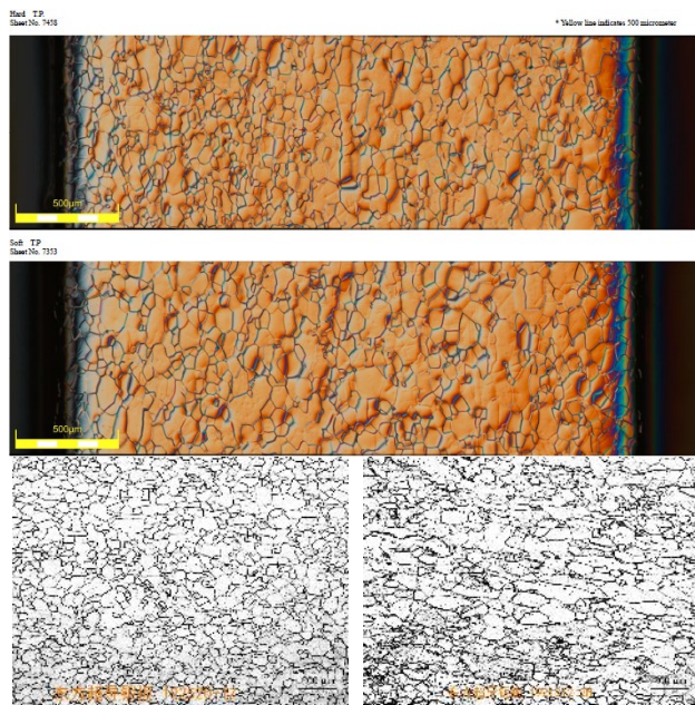
Figure 1: Micrograph of niobium material. Up: TD material. Bottom: NX material.
