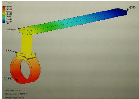
Figure 5: Temperature distribution of absorber with 35 W dissipated power.
