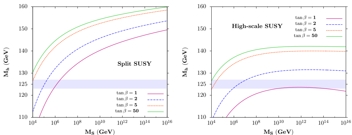
Figure 4. The value of M_h as a function of M_S for several values of \tan \beta = 1, 2, 5, 50 in the split SUSY (left) and high-scale SUSY (right) scenarios. From Ref. [4].
