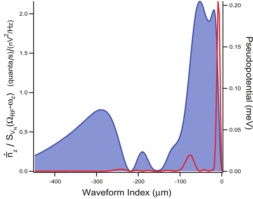
Figure 3. The ratio of the heating rate \dot{\bar{n}} (in quanta/s) to voltage noise spectral density S_{V_N}(\Omega_{\text{RF}} - \omega_z) , in units matching figure 8 of [13] (plotted in red). The shaded blue curve shows the trapping pseudopotential. Both quantities are plotted versus the distance from the junction center along z (figure 1(a)).
