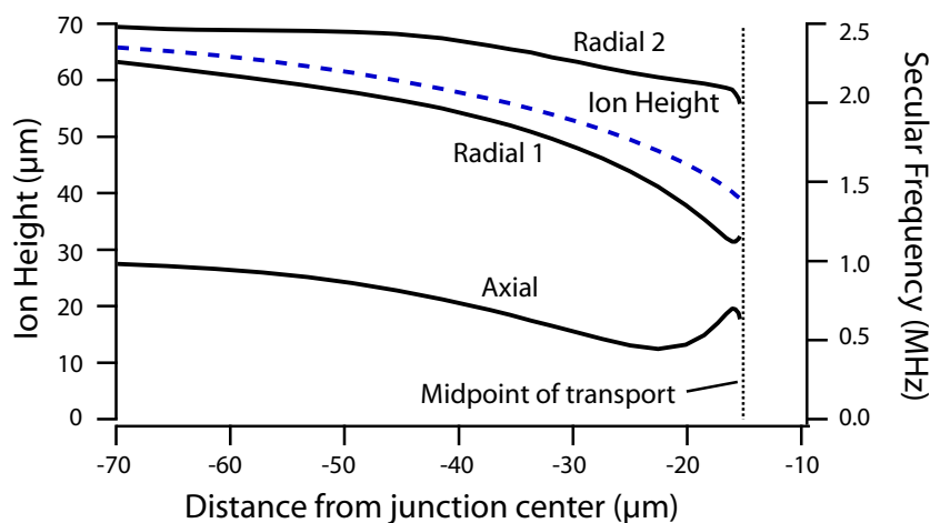
Figure 4. Calculated secular mode frequencies (solid) and ion height (dashed) for a waveform ( -z \rightarrow +x or -x ) designed for transport from one leg of the junction to the midpoint between the two legs. The potential forces the ion to circumnavigate the junction center at a 15 \mu\text{m} radius (see text).
