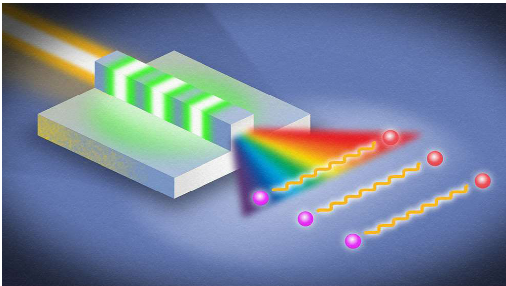
Figure 1. This artist rendition by researchers U. Javid and M. Osadciw in the lab of Qiang Lin at the Univ. of Rochester in New York depicts entangled photons .
