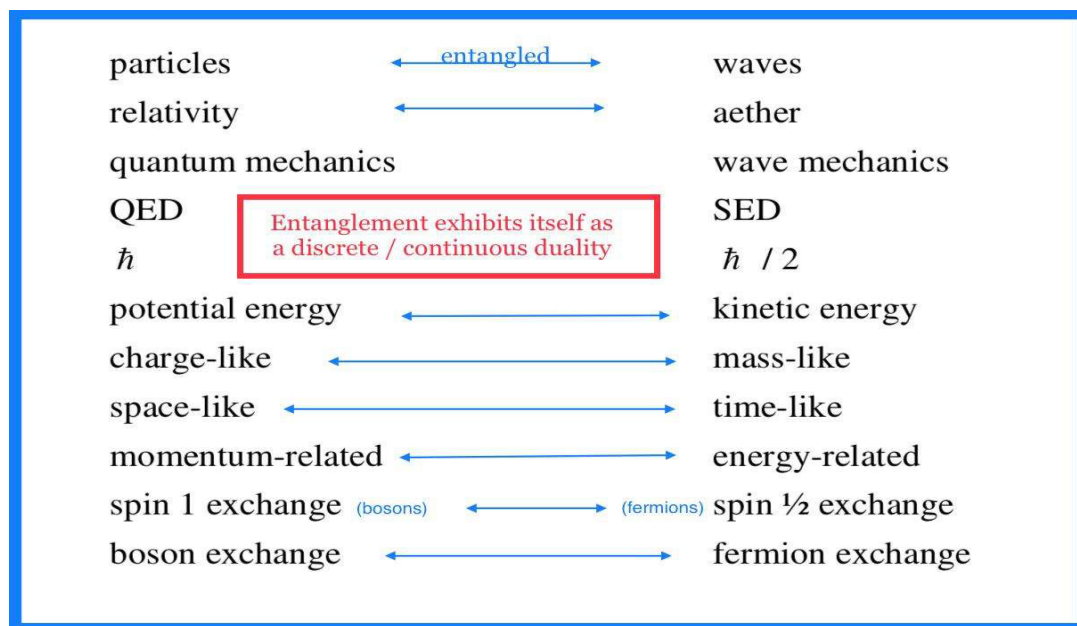
Figure 2. Fundamental physics depends on continuous and discrete approaches
