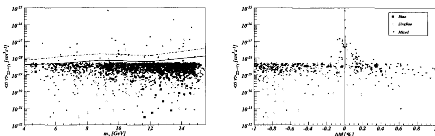
Figure 2: \langle\sigma v\rangle_{\chi\chi\rightarrow\gamma\gamma} with respect to the neutralino mass m_{\chi} (left panel) and \Delta M (right panel, see text for its definition) for several types of neutralinos. Solid lines are limit from the galactic center and the broken one from the halo.
