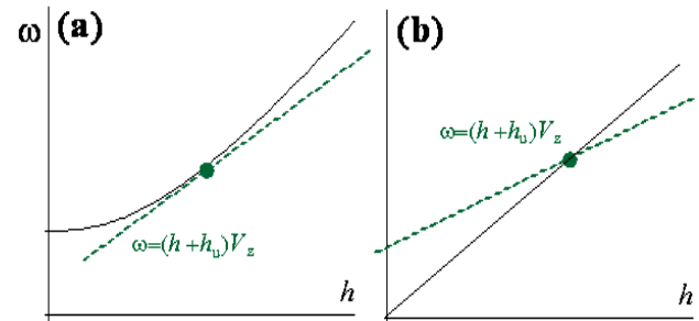
Figure 3: Dispersion diagrams in the regime of super-radiation of a wave packet propagating in a waveguide with a group velocity being equal to the electron velocity (a), as well as in the regime of the SASE amplification of a wave packet propagating in the free space with the speed of light (b).
