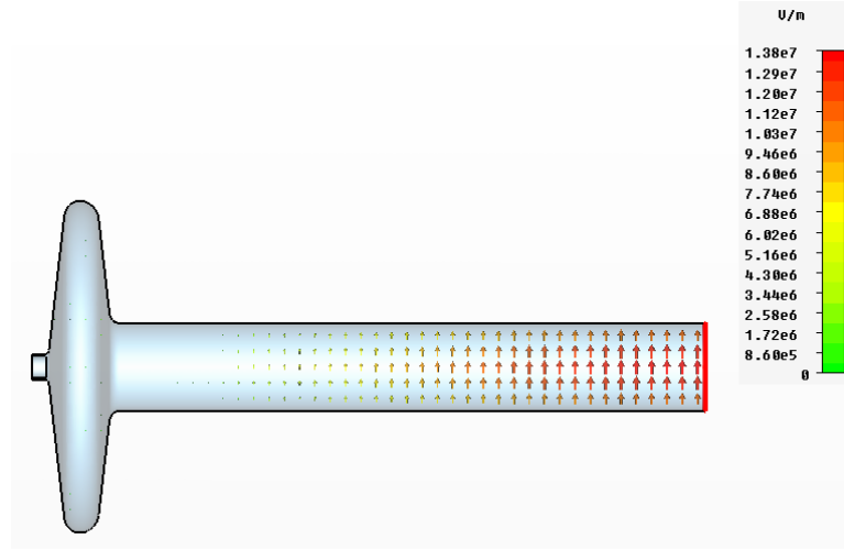
Figure 5.13: An example of the simulation result for the mode at 1.761 GHz. While this mode has a TM dipole mode profile in the cavity, this is essentially a mode of the beam pipe and, therefore, couples strongly to the ceramic-ferrite damper as measurements show. The existence of modes of the beam pipe is important to recognize in measurements of damping in both the gun and the five-cell cavity since they can be easily confused with modes of the cavity.
