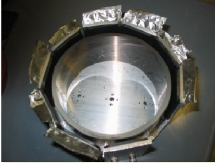
Figure 5.5: Experimental damper arrangement with glass insert.
