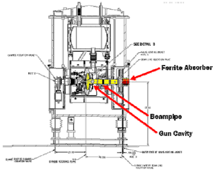
Figure 4.5: Schematic of gun inside of cryomodule with ferrite absorber attached.
