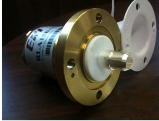
Figure 4.15: EIA connector used for mock FPC.
