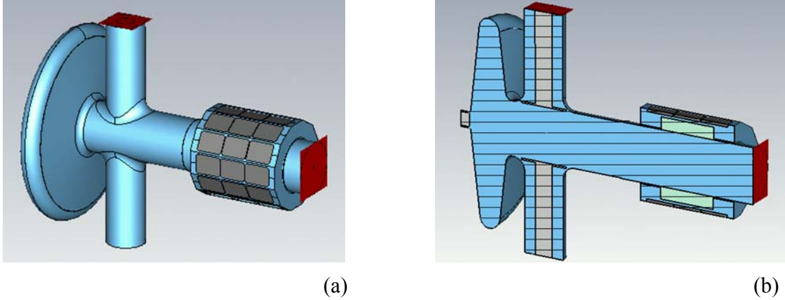
Figure 5.8: Model of the gun attached to the ceramic/ferrite damper in (a). In (b), a cutaway view of the model is shown, exposing the ceramic layer inside the ceramic/ferrite damper. Red boxes are waveguide ports through which energy can pass into and out of the structure.
