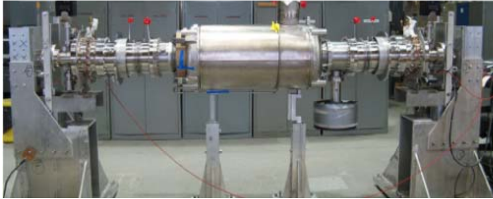
Figure 3.2: The ERL cavity string.
