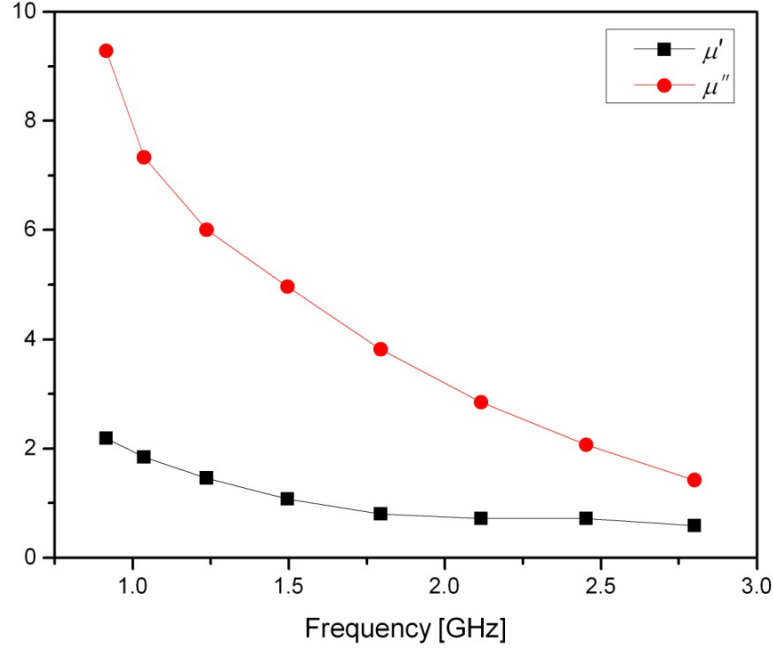
Figure 5.17: Complex permeability data as measured by Mouris and Hutcheon. \mu' is the real part and \mu'' is the imaginary part of the permeability.
