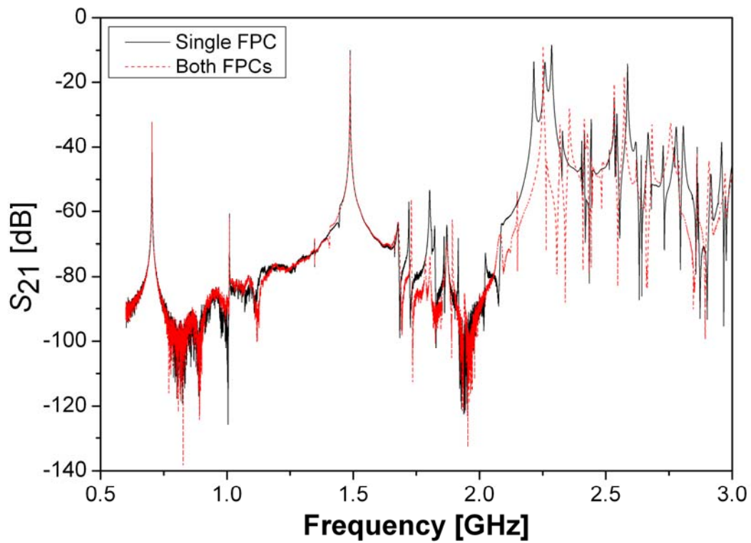
Figure 4.23: S_{21} measurements for configuration with single FPC and both FPCs inserted.
