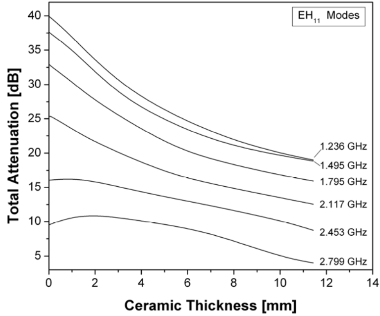
Figure 5.20: Total attenuation of EH_{11} modes of ceramic/ferrite damper for various frequencies.
