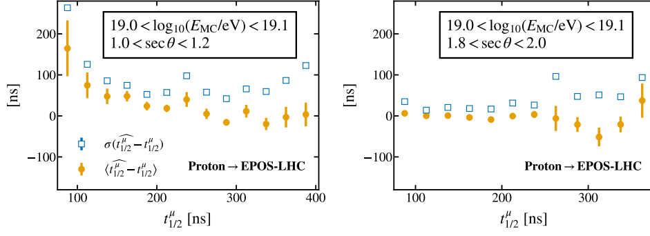
Figure 7: Mean and standard deviation of the difference between the risetime of the predicted muon signal \widehat{t_{1/2}^\mu} and the risetime of the true muon signal t_{1/2}^\mu for all the stations from events with the energies and zenith angles specified in the boxes.
