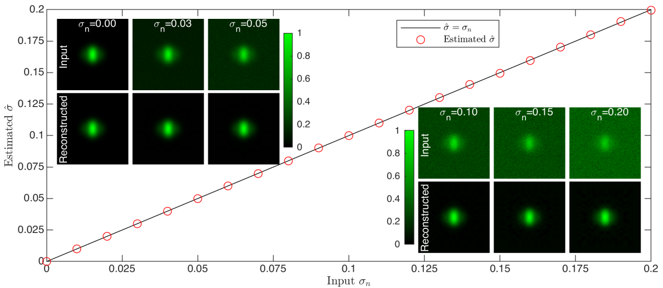
Figure 1: Mode decomposition and image reconstruction results. Gaussian noises with different levels (input \sigma_n ) are added to the same ideal beam (65% HG 0,0 , 20% HG 0,1 , and 15% HG 2,0 ) to obtain the input images. Using these images, the modal weights and \hat{\sigma}^2 are retrieved. The insets show the input and reconstructed images at different \sigma_n values.
