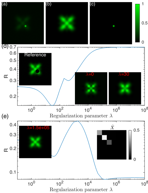
Figure 2: Modal analysis with different values of regularization parameter \lambda . Test beam (a) is the sum of an ideal beam (b), a diffraction pattern (c), and Gaussian noise with \sigma_n = 0.05 ; (d) Intensity difference R between the reconstructed image and reference image (top-left inset) as a function of \lambda . The two bottom-right insets are the reconstructed images with zero regularization ( \lambda = 0 ) and optimal regularization ( \lambda = 30 ), respectively. (e) Intensity difference R after the second iteration. The top-left inset is the reconstructed image with optimal regularization ( \lambda = 1.5 \times 10^5 ). The top-right inset shows the corresponding reconstructed weight matrix \hat{X} .
