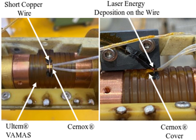
Fig. 2. Calibration setup with a short copper wire installed over a Cernox temperature sensor.
