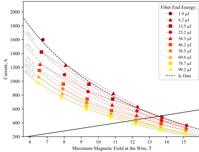
Fig. 5. Summary of laser-induced quench energy tests for BB-PIT wire at 4.2 K, with markers indicating the lowest Fiber End Energy sufficient to induce a quench at each magnetic field and current level.
