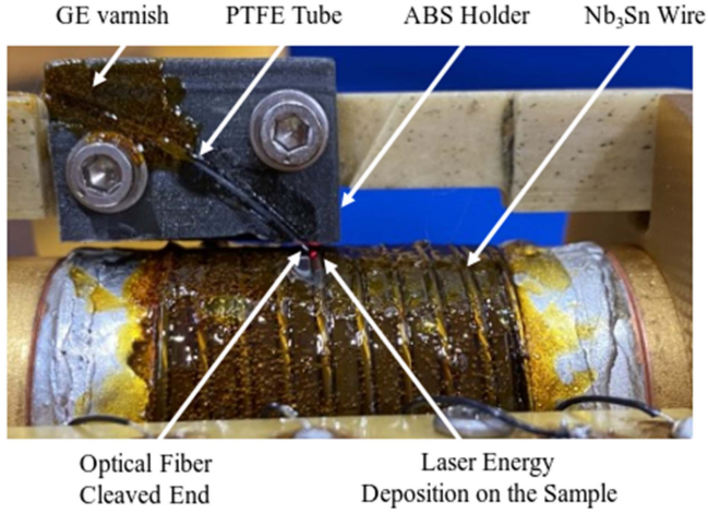
Fig. 1. Superconducting sample with optical fiber for laser-induced quench study.
