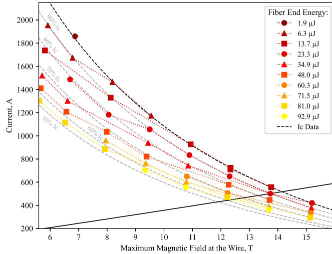
Fig. 4. Summary of laser-induced quench energy tests for RRP wire at 4.2 K, with markers indicating the lowest Fiber End Energy sufficient to induce a quench at each magnetic field and current level.
