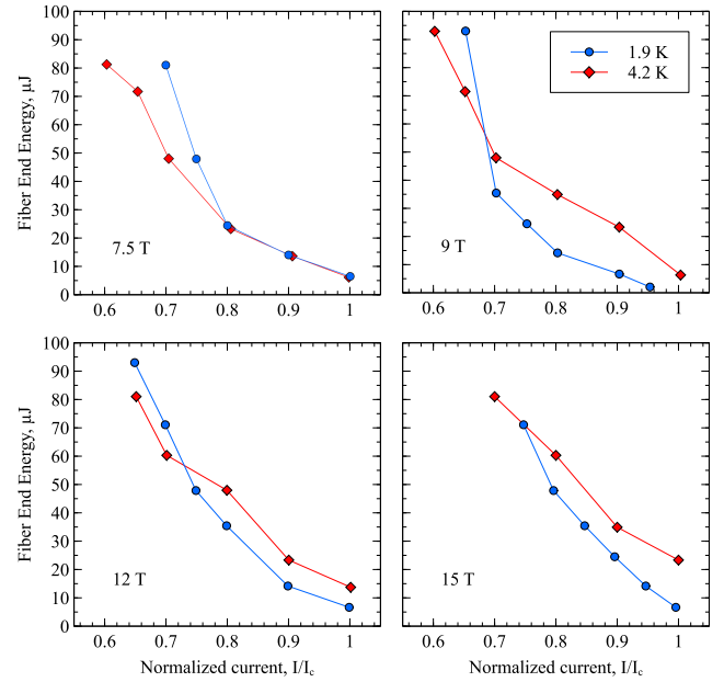
Fig. 6. Energy required to induce a quench of the RRP wire vs. normalized current at 1.9 K and 4.2 K at selected magnetic field levels.
