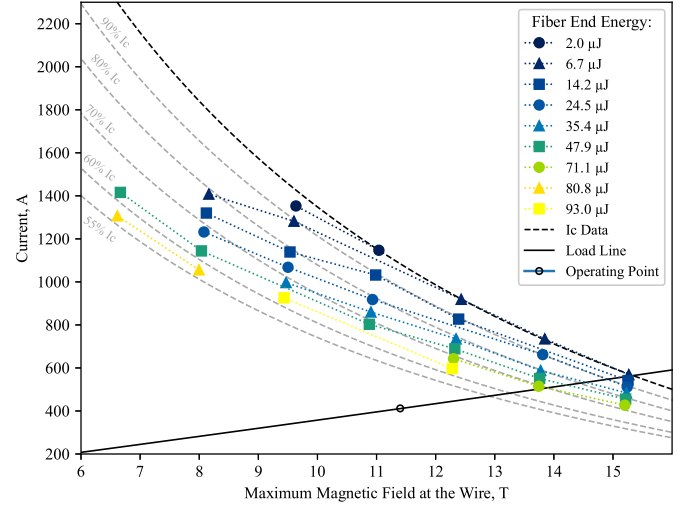
Fig. 3. Summary of laser-induced quench energy tests for RRP wire at 1.9 K, with markers indicating the lowest fiber end energy (see Section IV, subsection B) sufficient to induce a quench at each magnetic field and current level. Premature quenches occurred at as low as 1494 A at 6 T, so the test range was limited to 1500 A. The operating point of the MQXF magnet is indicated [15]. The percentage of the I_c , plotted in light grey, serves as a visual guide. The fiber end energy reported in the legend is the energy measured at the fiber output at room temperature. A previous calibration [7] suggested the absolute MQE would be 80% of this value (see Section IV).
