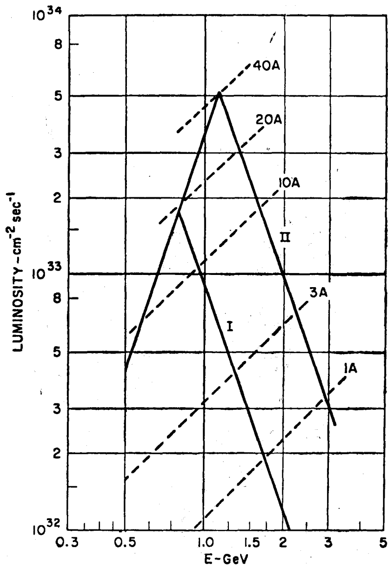
Fig. 5 Luminosity versus energy for Stage I and Stage II (solid curves). The dashed curves indicate the maximum luminosity which can be achieved with a given circulatory current.
