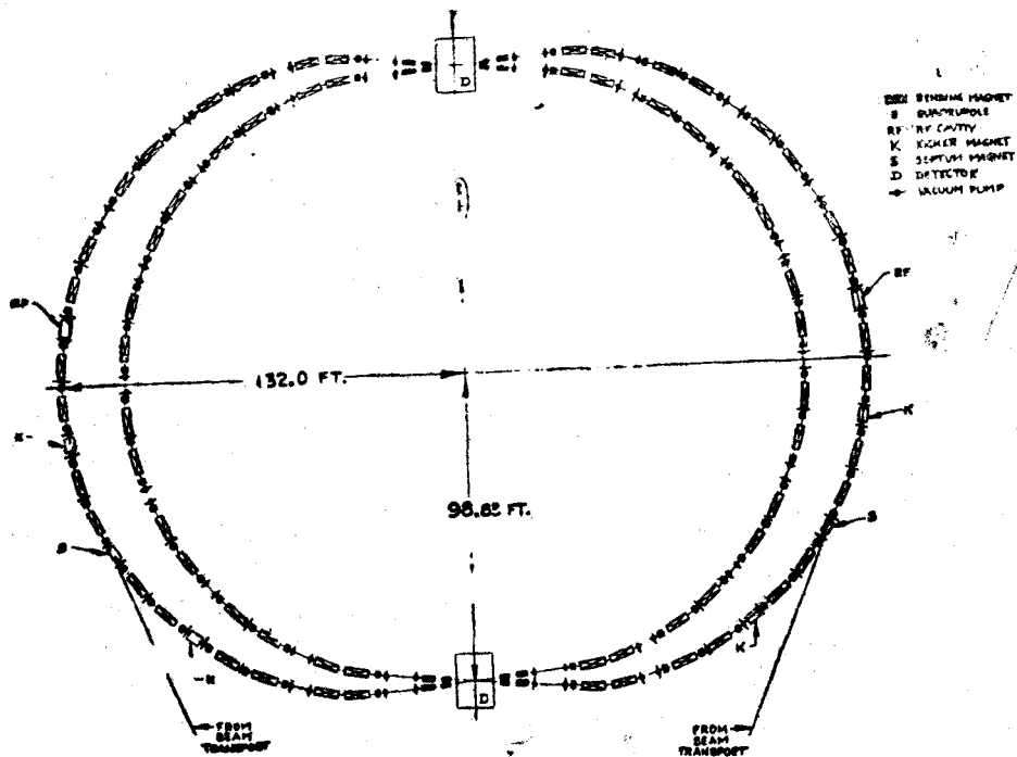
Fig. 1 Schematic of the double ring.
