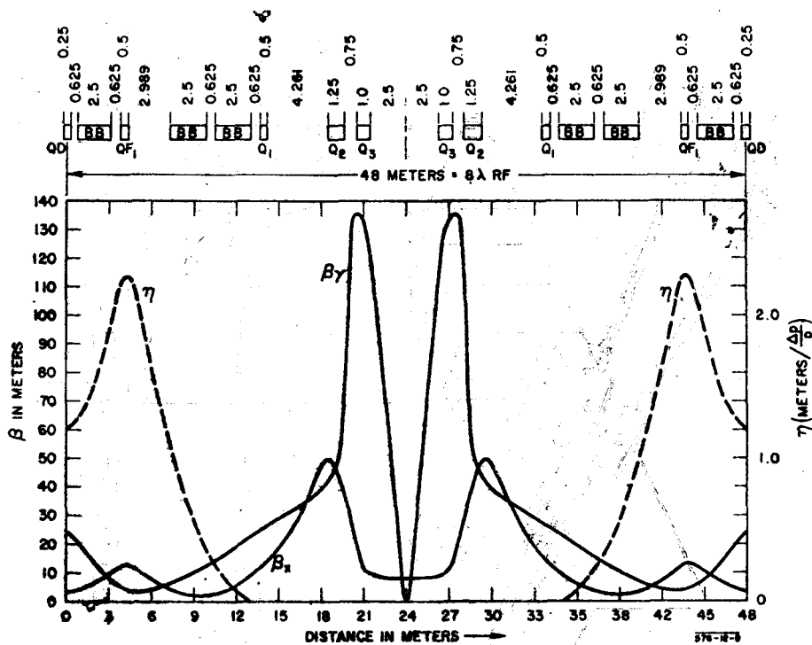
Fig. 3 Magnet lattice, \beta functions (left scale) and the equilibrium orbit of off-momentum particles ( \eta , right scale) in the low \beta orbit.
