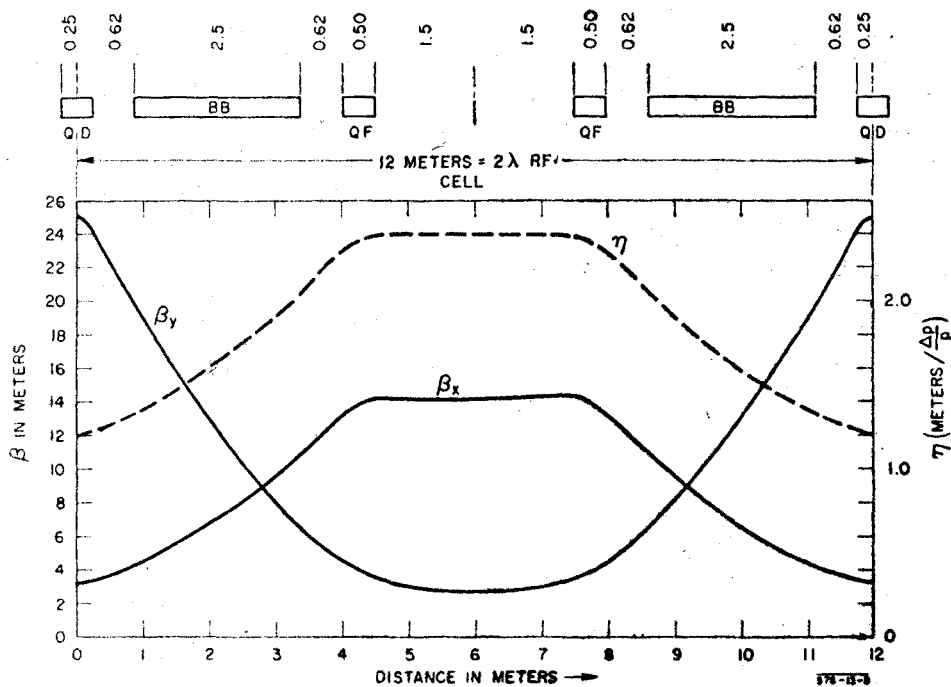
Fig. 2 Magnet lattice, \beta functions (left scale) and the equilibrium orbit for off-momentum particles ( \eta , right scale) in a standard cell.
