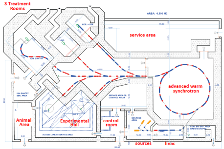
Figure 2: SEEIIST Layout.
