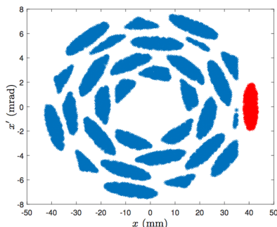
Figure 3: Multi-turn injection simulations from [7].
