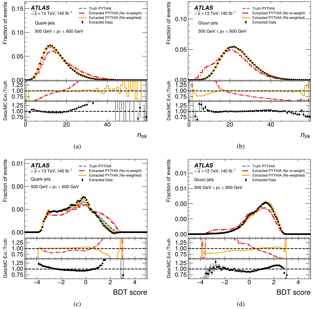
Fig. 3. (color online) The distributions of n_{\text{trk}} (a,b) and BDT score (c,d) in quark-jets (left) and gluon-jets (right) in the p_T range between 500 GeV and 600 GeV obtained from truth Pythia (dashed line), extracted Pythia before re-weighting (dash-dotted line) and after re-weighting (solid line), and extracted data (dots) are shown in the top panel. The middle panel shows the ratio of extracted Pythia to truth Pythia. The bottom panel shows the ratio of extracted data to extracted Pythia after re-weighting.
