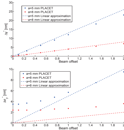
Figure 6: Linear approximation and PLACET simulations of the orbit displacement (top) and beam size growth (bottom) as a function of the beam offset for a=5 mm and a=8 mm.
