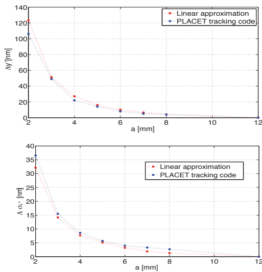
Figure 5: Linear approximation and PLACET tracking simulations of the orbit displacement (top) and beam size growth (bottom) at the IP as a function of a and 1 mm beam offset.
