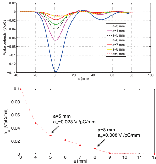
Figure 4: Wakepotential (top) and average transverse dipole kick as a function of a (bottom).
