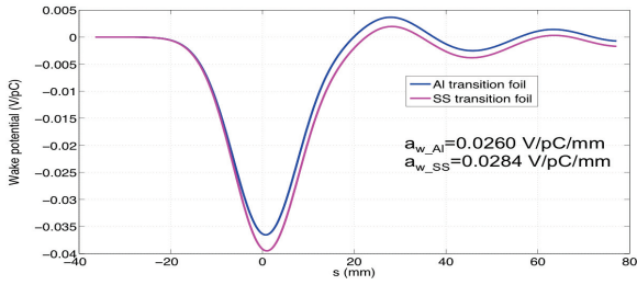
Figure 3: SS and Al transition foil wakepotential comparison.
