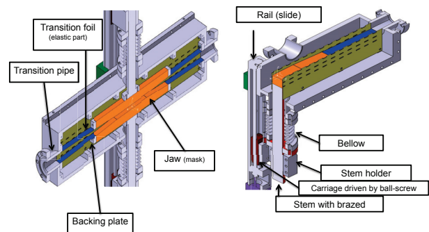
Figure 1: Detailed 3D mechanical design.
