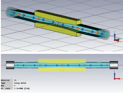
Figure 2: CST PS realistic model of the rectangular vertical tapered collimator.
