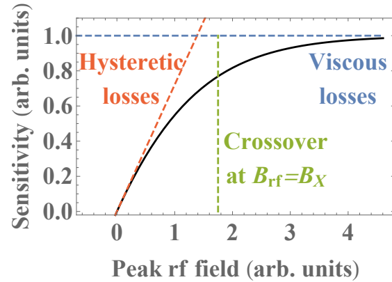
Figure 4: Illustration of the sensitivity of the residual resistance due to trapped magnetic flux as a function of the RF field strength, with crossover between the low-field linear regime and the high-field constant regime. Originally published in [22].
