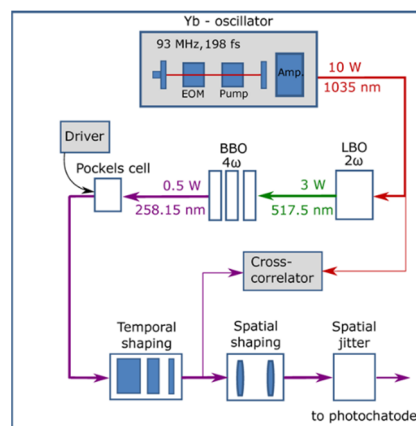
Figure 3: Schematic layout of the laser system able to generate 4 th harmonic pulses with a proper time and spatial profile.
