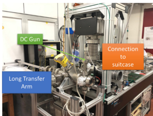
Figure 2: Picture of the HV DC gun installed at INFN LASA before its installation in the new Laser Laboratory.
