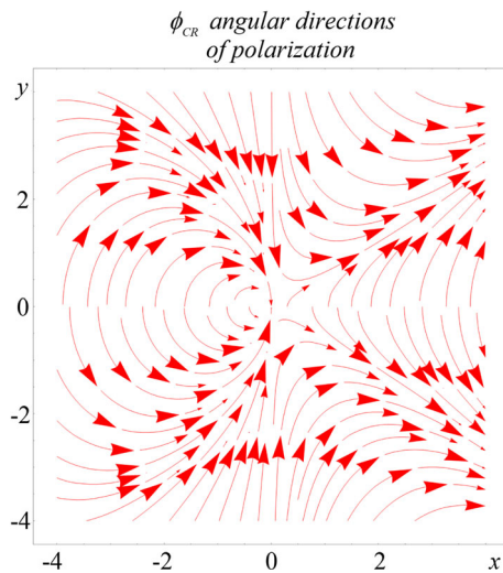
Fig. 5 The map of angular directions of polarisation CR for photons with positive helicity \Lambda = 1 (for \Lambda = -1 the directions will be opposite) generated by 10 MeV electrons channeled along the \langle 100 \rangle axes in Si for selected transverse plane is shown in Fig. 1
