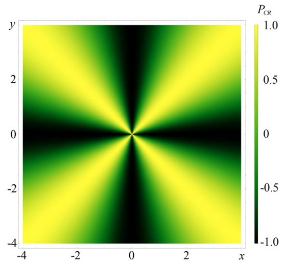
Fig. 4 Arbitrary contour plot of the degree of polarisation for CR by 10 MeV electrons channeled along Si \langle 100 \rangle for a selected transverse plane shown in Fig. 1
