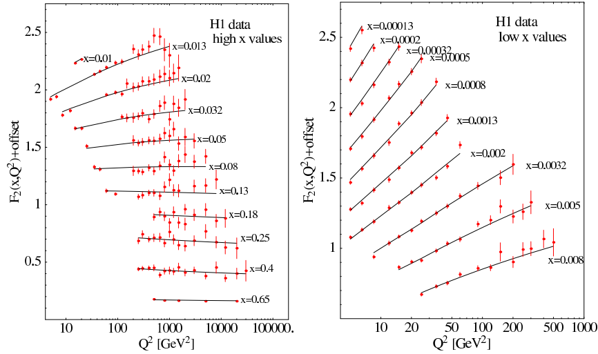
Fig. 2. Left: Approximate scaling at moderate x . Right: Pronounced evolution for smaller x . Data from the H1 experiment at HERA.
