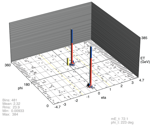
Fig. 6. Jet pair at a hadron collider. Event recorded by the DØ experiment at Fermilab.
