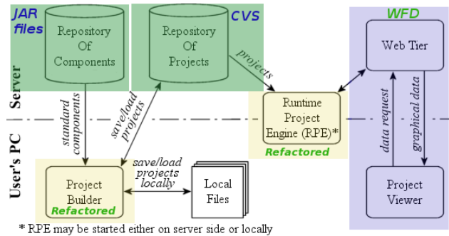
Figure 1: DnD Architecture.
