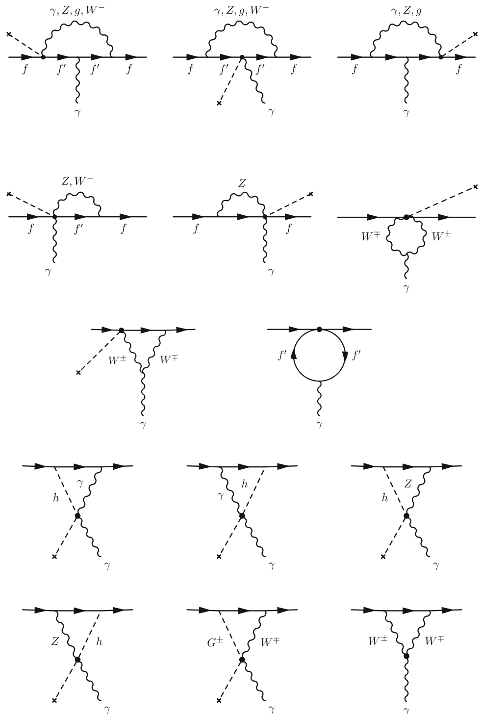
Fig. 13 1PI diagrams contributing to the \bar{\psi}\psi\gamma 3-point function. Notice that the diagram with the lepton loop exists only for external up-type quarks and leptons
