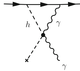
Fig. 3 Representative diagram giving a contribution of the H^2 F^2 class of operators to the dipole operators
