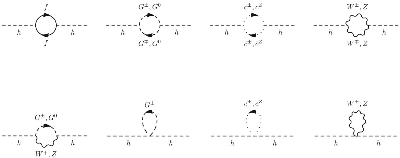
Fig. 10 Diagrams contributing to the Higgs 2-point function
