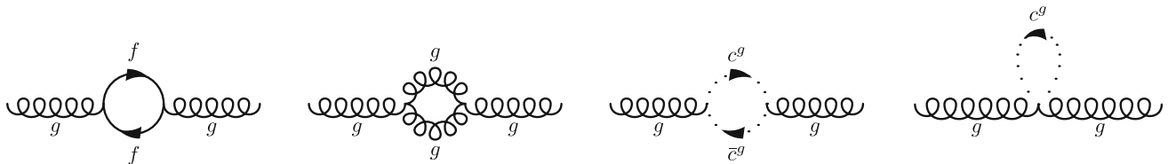
Fig. 11 Diagrams contributing to the gluon 2-point function
