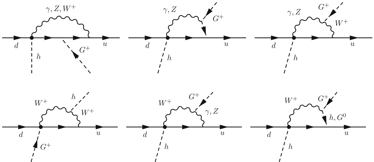
Fig. 17 1PI diagrams contributing to the udhG^+ 4-point function. We only show the contribution of the down-type dipole. Furthermore, additional diagrams can be generated by exchanging h \leftrightarrow G^+
