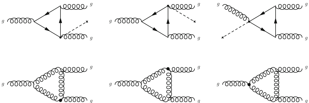
Fig. 12 1PI diagrams contributing to the ggg 3-point function. Of course, there are also diagrams with only two propagators for both the insertion of the Weinberg and the dipole operator, but we find that these
