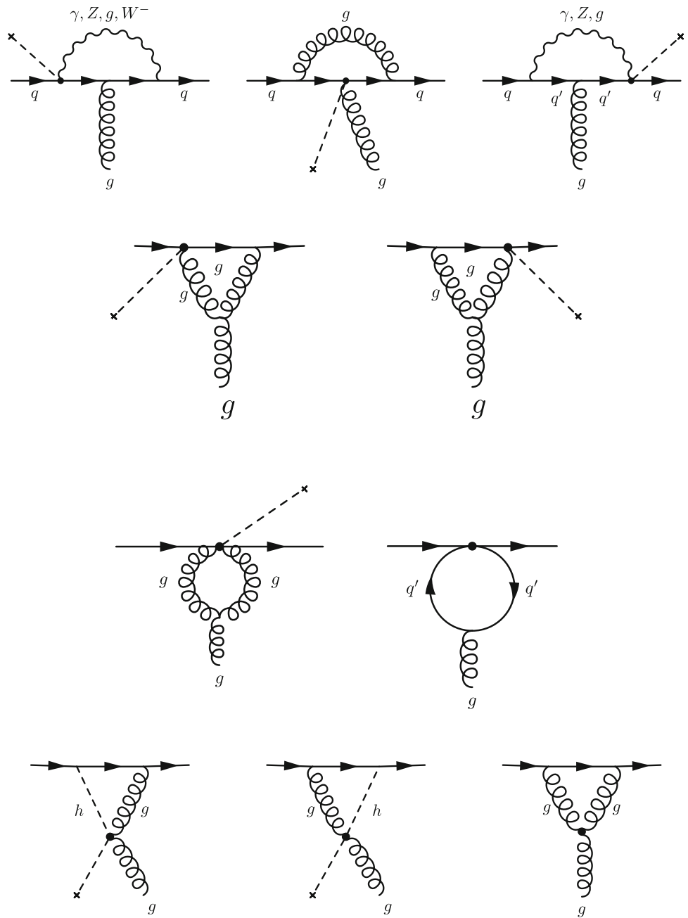
Fig. 14 1PI diagrams contributing to the \bar{q}qg 3-point function
