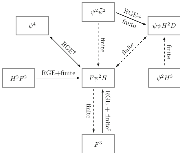
Fig. 2 Contributions to the operators entering the dipoles. Operators connected with solid arrows enter the RGEs, while dashed arrows describe purely finite effects. The † indicates that the operator O_{lequ}^{(1)} is not included in the \psi^4 class here. Interestingly, we find that the others operators in this class only enter via the RGE, generating no rational terms. The ‡ shows that the operator O_{\tilde{W}} gives only rational terms
