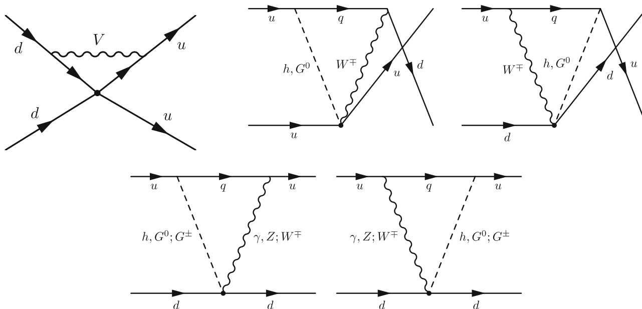
Fig. 15 1PI diagrams contributing to the udud 4-point function. For diagrams contributing to the self-renormalization, we show only one representative diagram, all the others can be obtained by connecting all possible pairs of external fermions with the internal vector. The other
