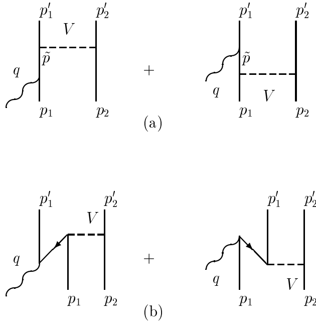
Figure 5.3: (a) Relativistic Born diagrams, (b) negative-energy components of the relativistic Born diagrams.
