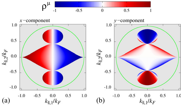
Figure 7. Spin polarization of the surface states at the (101) surface of a C_{4v} point group NCS with r = 0.25 . Panels (a) and (b) show the spin polarization along the x - and y - axes of the crystal, respectively. The z -spin polarization is vanishing. The energy of the states is shown in figure 6(b). Figure adapted from [85].
