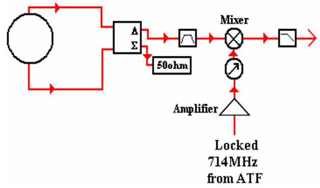
Figure 4: Schematic of BPM signal processor.
