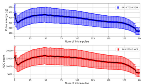
Figure 1: Single-shot SASE3 FEL pulse energies measured by the MCP and XGM for each X-ray pulse of a train of 200 pulses.
