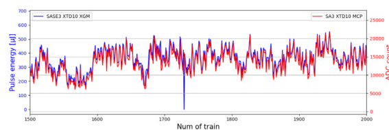
Figure 2: SASE3 FEL pulse energy measured by the MCP and XGM over 6000 consecutive pulse trains.
