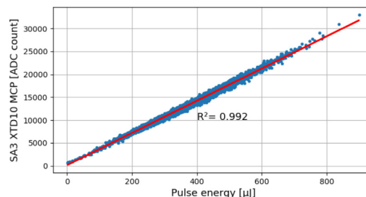
Figure 3: Correlation plot of average MCP and XGM signals.
