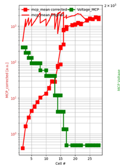
Figure 4: Dependence of the MCP pulse energy signal (red squares) and the MCP voltage (green squares) on the number of active (closed) SASE 2 undulator cells. The uncorrected raw data (red line without symbols) is shown for reference where the MCP gain was changed.
