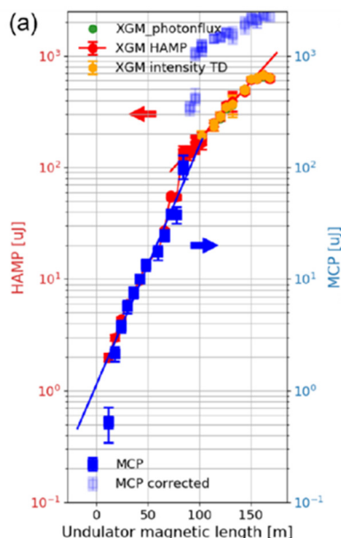
Figure 5: The dependence of corrected MCP pulse energy (blue), corrected HAMP (red) and XGM photon flux (in green) and the mean value of the pulse-resolved XGM data on SASE 2 undulator length.
