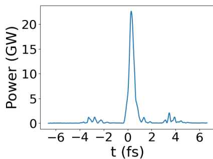
Figure 9: Power profile of the 700 eV FEL pulse at the exit of the second stage.
