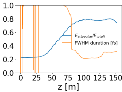
Figure 3: The change of pulse duration and contrast along the undulator.
