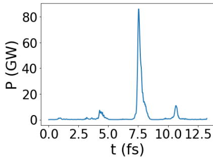
Figure 4: Power profile of the 6 keV FEL pulse at the position of 130 m.
