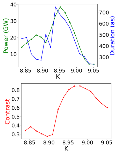
Figure 8: Scanning of the undulator strength of the second stage.
