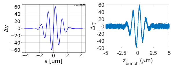
Figure 2: Energy modulation induced by the laser, obtained by theoretical analysis (left) and three-dimensional simulation (right). The bunch head is to the right.
