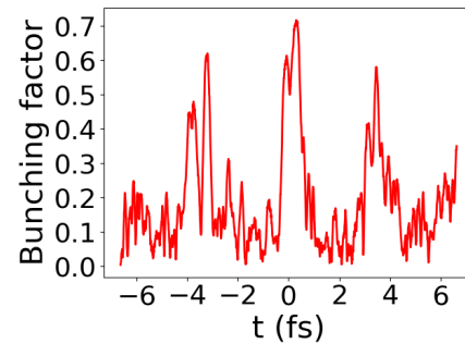
Figure 7: Bunching factor distribution at the exit of the first stage.
