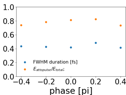
Figure 10: CEP stability analysis of the chirp-taper scheme at 700 eV.
