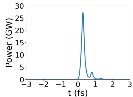
Figure 12: Power profile of the 700 eV FEL pulse obtained with the ESASE scheme.
