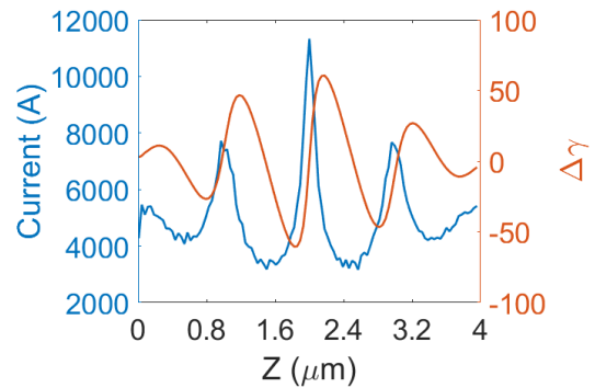
Figure 11: Energy modulation induced by the laser and current profile of the electron beam for the ESASE scheme.
