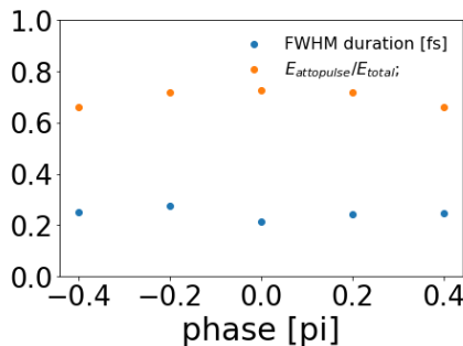
Figure 5: CEP stability analysis of the chirp-taper scheme at 6 keV.
