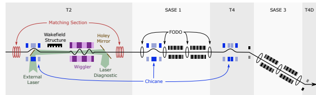
Figure 1: Schematic layout of the ASPECT project.
