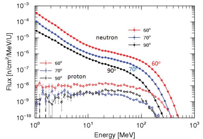
Figure 4: Energy spectra of neutrons and protons at the three activation detector locations.
