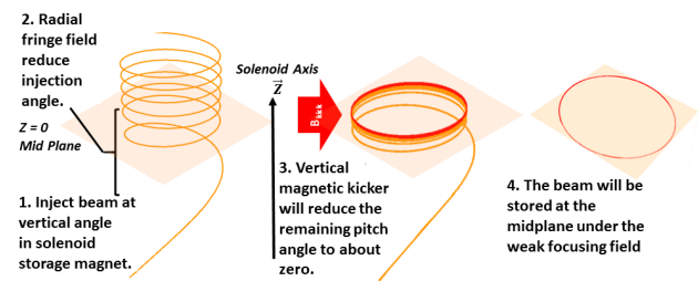
Figure 1: Layout of three-dimensional spiral injection scheme.
