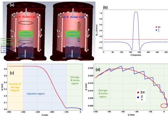
Figure 5: (a) Two models of the magnetic kicker. (b) Magnetic field profile for the 2\pi and \pi/6 kicker model. The required magnitude of magnetic field increase in the case of \pi/6 kicker model due to a limited region. (c) The pitch angle starting from the injection point to the storage region as a function of the vertical position ( Z ). (d) Pitch angle in the kicker and storage region.
