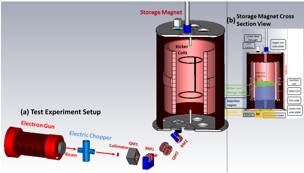
Figure 2: (a) A diagram showing the 3D schematic of spiral injection test experiment. (b) The schematic of the storage magnet with monitors and reference trajectory.
