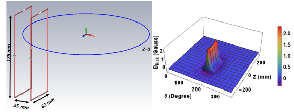
Figure 6: Left: Optimized \pi/6 kicker model. Right: Magnetic field map in radial and vertical directions. The exciting current of the coil was set to 10 A.
