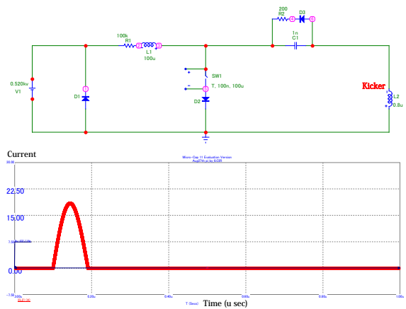
Figure 7: Top: The schematic electronic circuit for the pulsed magnetic kicker. Bottom: The pulsed current through kicker coil.
