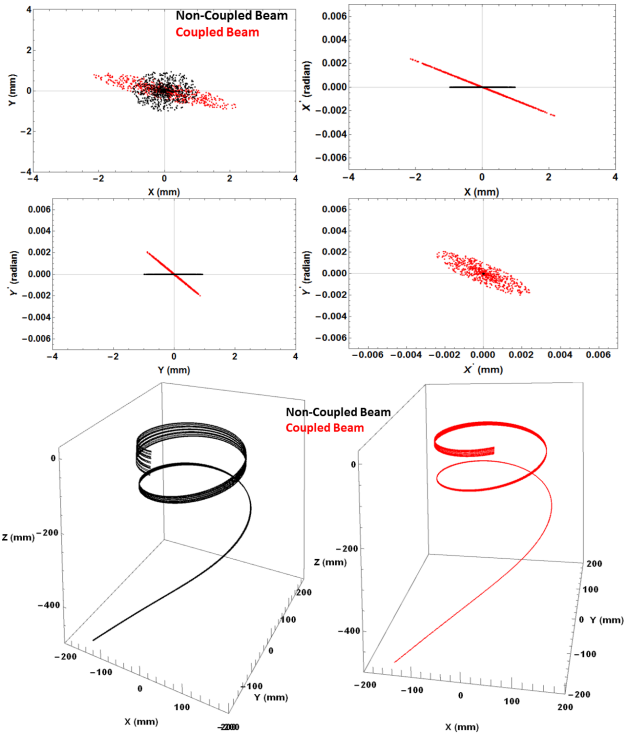
Figure 3: The above four plots are the required phase space at the matching point ( Z = -500 mm). The black points show the beam phase space without coupling and red points show with coupling. Bottom two plots are showing the beam injection with and without coupled beam.
