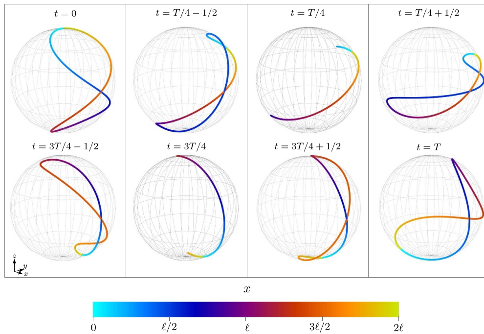
Figure 2. Time evolution of the breather solution with initial data (5.31) II: spatial dependence of \mathbf{u}_0(x, t) at eight instances of time t measured in the ‘period’ time T \approx 11.83 , with colours indicating the position x according to the legend on the bottom. Note that at t = T/4 and t = 3T/4 , when \mathbf{u}_0(x, t) is not differentiable at two points, \mathbf{u}(x, t) traces its image exactly twice as x goes from 0 to 2\ell . The plots only show one such tracing. By comparing t = 0 and t = T one sees that the image of \mathbf{u} is not periodic in time, in contrast to the pole and energy evolution (see figures 1 and 3). The time evolution of \mathbf{v}_0(x, t) is the reflection of \mathbf{u} in the xz -plane. The orientation of all plots is the same and indicated by the coordinate system in the bottom left corner. Note that we plot \mathbf{u}_0(x, t) instead of \mathbf{u}(x, t) to avoid obfuscating the breather behaviour by the action of the global rotation \mathbb{R} .
