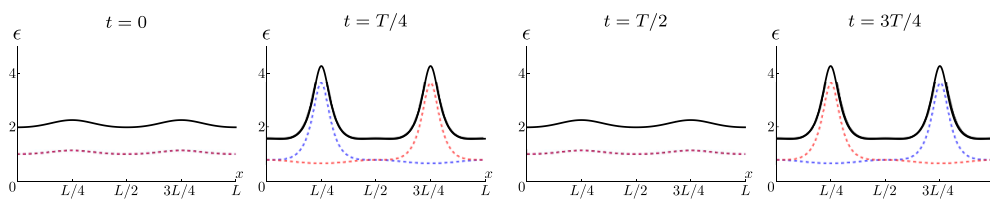
Figure 3. Time evolution of the breather solution with initial data (5.31) III: energy density at four instances of time t . At each time t , the total energy density \epsilon(x, t) = \epsilon_u(x, t) + \epsilon_v(x, t) and the individual energy densities \epsilon_u(x, t) (red) and \epsilon_v(x, t) (blue) (5.33) of the \mathbf{u} - and the \mathbf{v} -channels are shown. The plots illustrate that the total energy density \epsilon(x, t) is periodic with period T/2 \approx 5.916 , but the \mathbf{u} - and \mathbf{v} -channel energy densities are periodic with period T \approx 11.83 only. At t = T the energy densities are exactly the same as at t = 0 .
