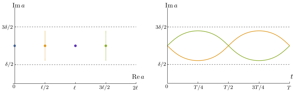
Figure 1. Time evolution of the breather solution with initial data (5.31) I: evolution of the poles. The left plot shows the location of the four poles a_1 (blue), a_2 (purple), a_3 (yellow), and a_4 (green) at t = 0 . In addition, the coloured shadow indicates the path the poles trace as time evolves, showing that a_1 and a_2 are stationary, whereas a_3 and a_4 oscillate vertically. The right plot shows the imaginary part of the two moving poles during a full period from t = 0 to t = T \approx 11.83 .
