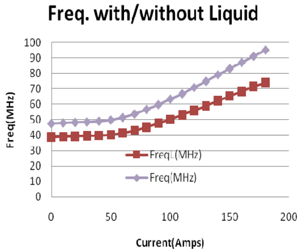
Fig. 9: Resonant frequency of the model cavity as a function of bias solenoid current using Toshiba M4C ferrite. The blue points are without dielectric liquid and the red points are with the cavity filled with dielectric liquid. These data are for Dow Corning 561 Silicon Transformer Liquid.
