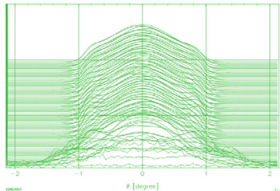
Fig. 11: The same conditions as figure 10, but with an added second-harmonic RF. The total ring voltage is 0.8MV with second harmonic 0.3MV. The effect of bunch flattening is visible.
