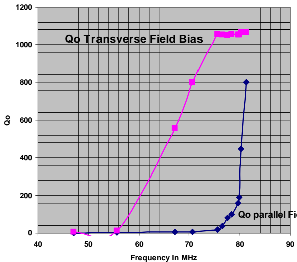
Fig. 5: Comparison of Q_0 as a function frequency for a garnet core for orthogonal (magenta) and for parallel (blue) biasing.
