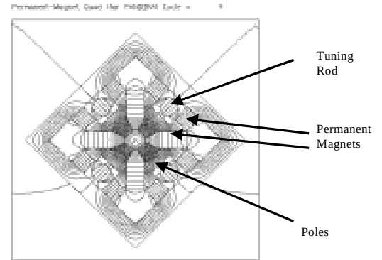
Fig. 3. Wedge quadrupole cross section showing the poles, magnet material and tuning rods. The field lines are also shown in this plot.
