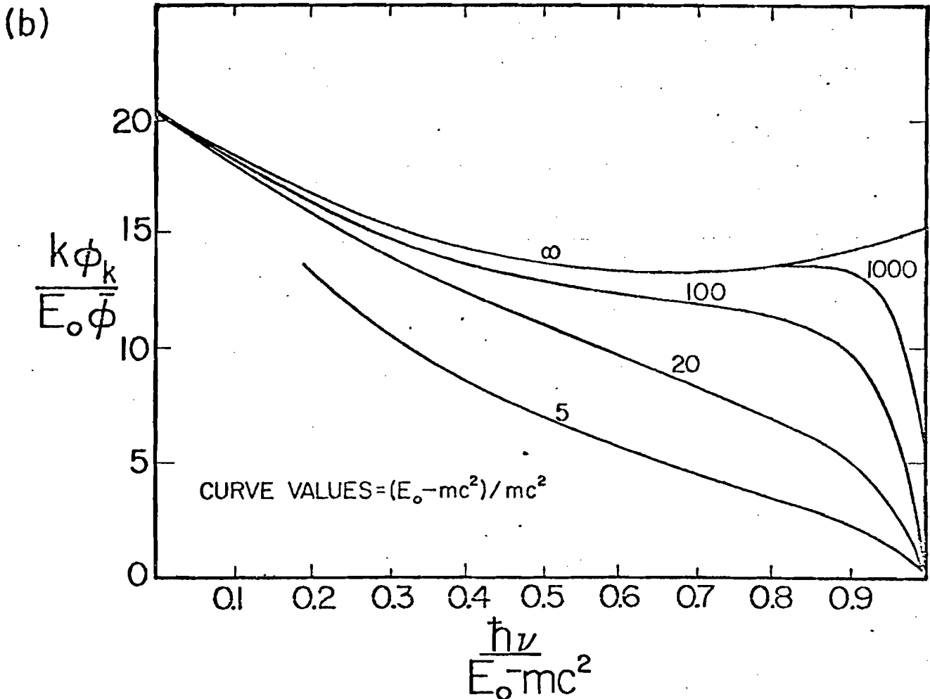
CALCULATED BREMSSTRAHLUNG INTENSITY AS A FUNCTION OF h\nu / (E_0 - mc^2) FOR LEAD
