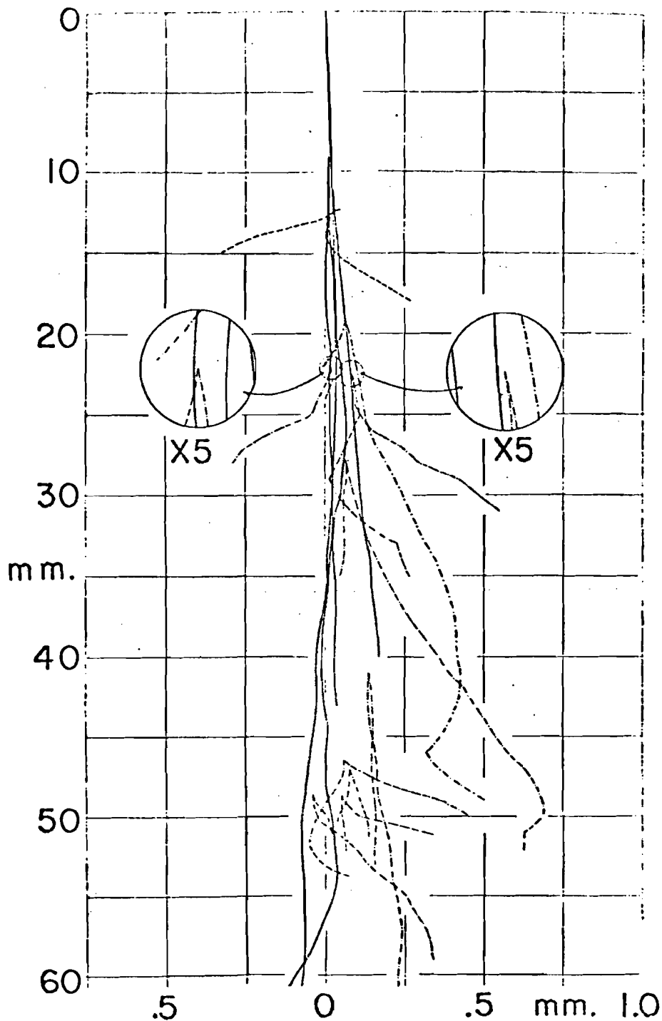
Hand-drawn drawing of the tracks in a cascade shower, initiated by an 10^8 GeV photon. Two radiation lengths of the shower development are shown. Note the factor of 20 difference in the horizontal and vertical scales. Particle tracks eventually disappear as they pass out of the plane of the photographic emulsion. (After G. H. Hooper, D. L. King, A. H. Morrish, Canadian Journal of Physics, 29, 559 (1951))
