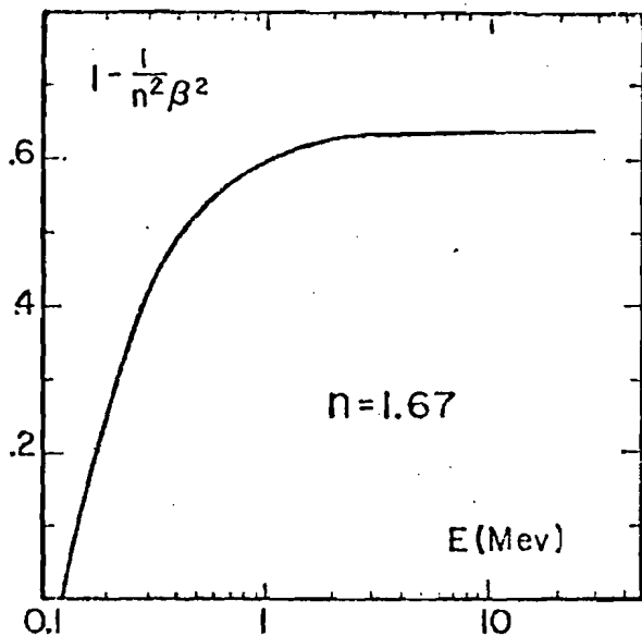
CERENKOV FACTOR vs ELECTRON ENERGY
