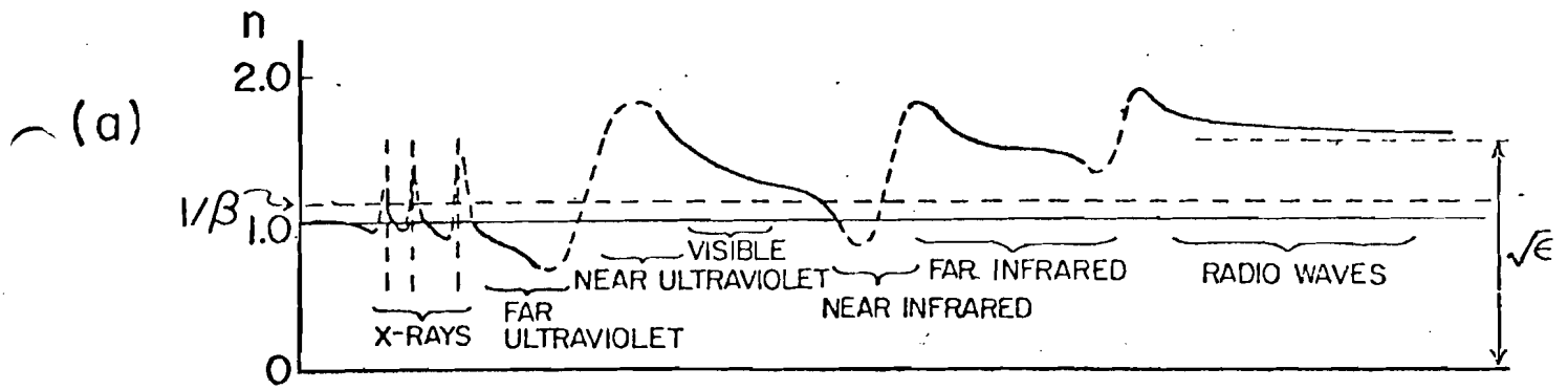
SCHEMATIC DISPERSION CURVE FOR OPTICAL MEDIA (after Jenkins and White, Fundamentals of Optics, p487 (3rd. Ed)).
