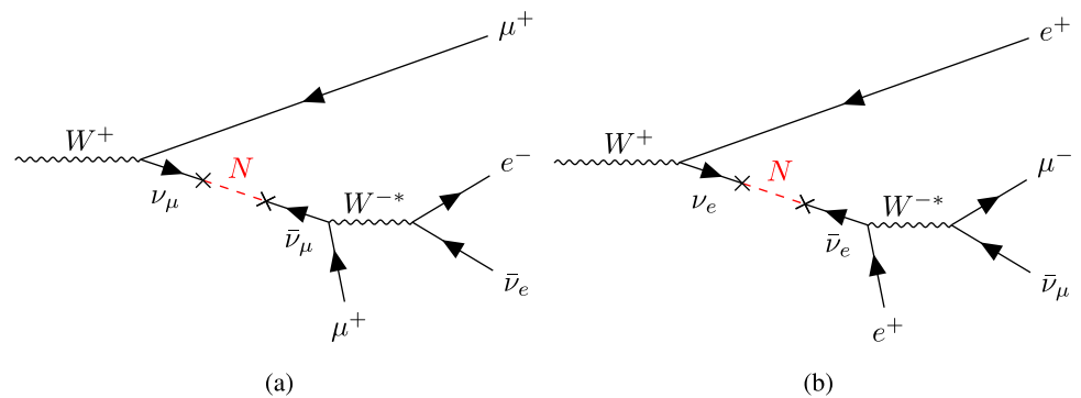
Fig. 1 Feynman diagrams for heavy neutral lepton ( N ) production and decay in the channels originating from: (a) HNL– \nu_\mu mixing and \mu^+ e^- \bar{\nu}_e decay of the heavy lepton, and (b) HNL– \nu_e mixing and e^+ \mu^- \bar{\nu}_\mu decay of the heavy lepton. Only lepton-number-violating processes are considered
