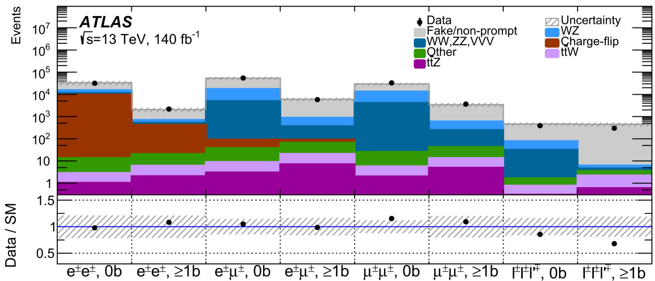
Fig. 2 Comparison between the data and estimated background at preselection level. Events entering the SRs defined in Sect. 5 are vetoed. The events are classified in terms of the number of leptons and their flavours, as well as the number of b -jets. The \ell^\pm \ell^\pm bins have a \geq 2 signal leptons selection, with no requirement on the number of base-
