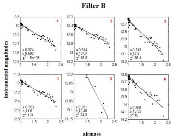
Figure 3. For six stars, measurements were made during a single clear night at different zenith angles (and thus different amounts of airmass between the star and the telescope) and a linear function was fitted to the results. By extrapolating the function to zero, one can obtain the instrumental brightness of the stars unaffected by atmospheric conditions and thus, by comparison with the catalog, calibrate the absolute response of the telescope to starlight.
