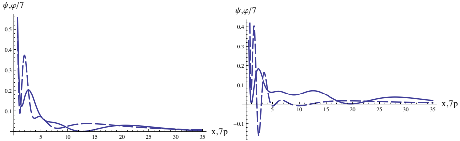
Fig. 5. Radial partners under Bessel transform. \psi (full lines) and \varphi (dashes). Left: Fourier-positive case \psi = e^{-\frac{x}{2}}(3.6096 - 6.7462x + 4.8826x^2 - 1.6141x^3 + 0.28086x^4 - 0.027009x^5 + 0.00145x^6 - 0.000042169x^7 + 5.63539 \cdot 10^{-7}x^8) . Right: non-Fourier-positive case \psi = e^{-\frac{x}{2}}(2.49362 - 6.84573x + 6.76697x^2 - 3.04127x^3 + 0.723816x^4 - 0.0959944x^5 + 0.00705616x^6 - 0.000265057x^7 + 3.93896 \cdot 10^{-6}x^8) . For graphical reasons, the figure actually shows \varphi(p/7)/7 .
