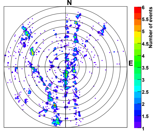
Figure 7.30.: Sky-map of the remaining background triggers after applying the dynamic T3-algorithm.
