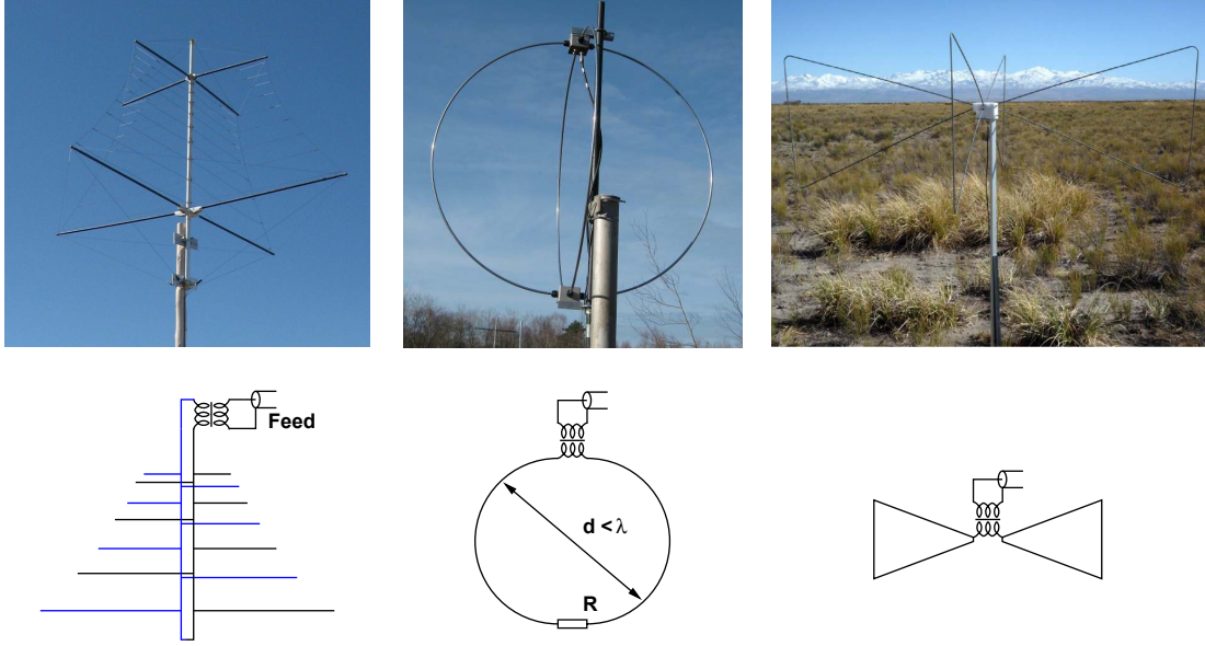
Figure 3.2.: Top: Pictures of the antenna candidates. Bottom: Internal antenna schematic, all antennas feed the coaxial cable via balanced-unbalanced transformers. a) Wired LPDA b) SALLA c) Butterfly antenna
