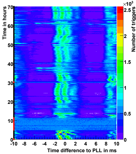
Figure 7.19.: Long term measurement of the periodic background relative to the PLL prediction. When PLL is not locked, the vertical axis is red.
