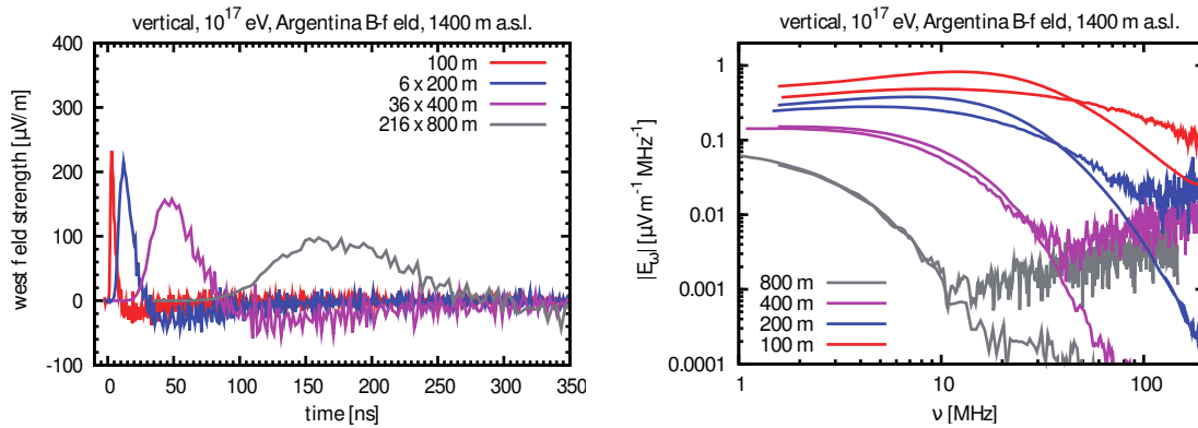
Figure 2.5.: REAS3-simulation of the radio pulse from an air shower. Left : East-west polarization of the time-dependent E-Field at different distances. Right : Signal spectrum comparing REAS3 (bold lines) and MGMR (thin lines) simulations [36].
