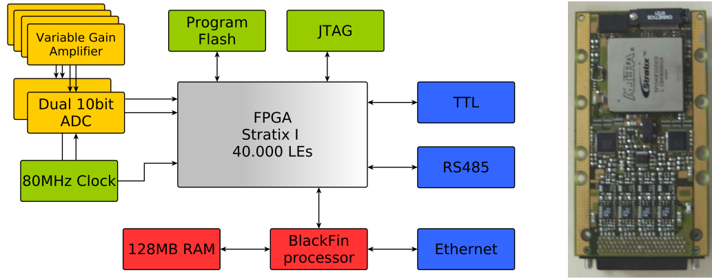
Figure 3.9.: Left: Block diagram of the prototype trigger hardware: Yellow blocks show the two analog channels, interfaces to the exterior are colored blue, the processor devices are red, and auxiliary units green. Right: Corresponding picture of the printed circuit board (PCB).
