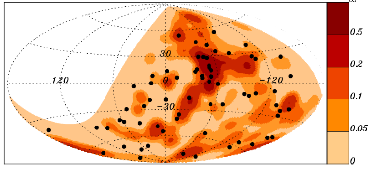
Figure 2.2.: Sky-map in galactic coordinates of AGNs of the Swift-BAT catalogue smoothed with a resolution of 5^\circ plotted in reddish color , and cosmic rays with energies above 5.5 \cdot 10^{19} \text{ eV} plotted as black points . An accumulation of events from the Centaurus A region is visible [9].
