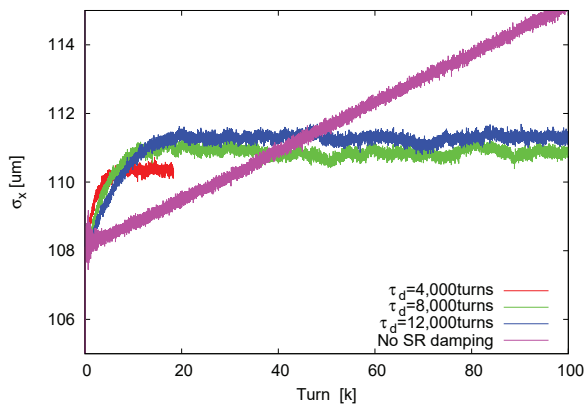
Figure 3: Equilibrium electron horizontal beam size as function of the radiation damping time.
