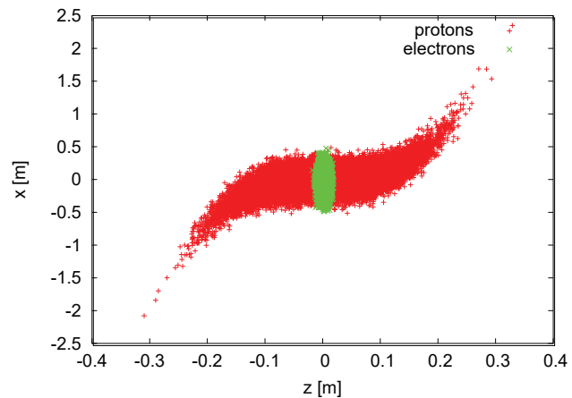
Figure 1: Electron and proton bunch profiles in the head-on frame.
