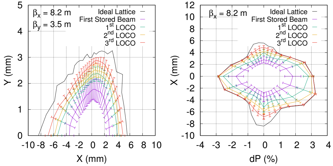
Figure 2. The on- and off-momentum dynamic apertures at different commissioning stages. The averages are connected by solid lines and the error bars are shown in dashes.
