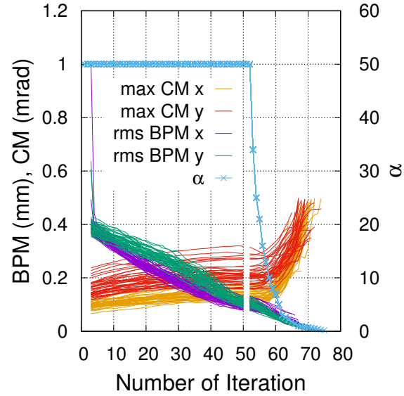
Figure 1. The change of the closed orbits and corrector strengths in the first BBA step. Before the iteration number 50, the BPM reading values decrease as the new BPM offsets are updated closer toward quad centres. After that, the BPM readings continue to decrease but the corrector strengths begin to increase rapidly in line with the decreasing \alpha .
