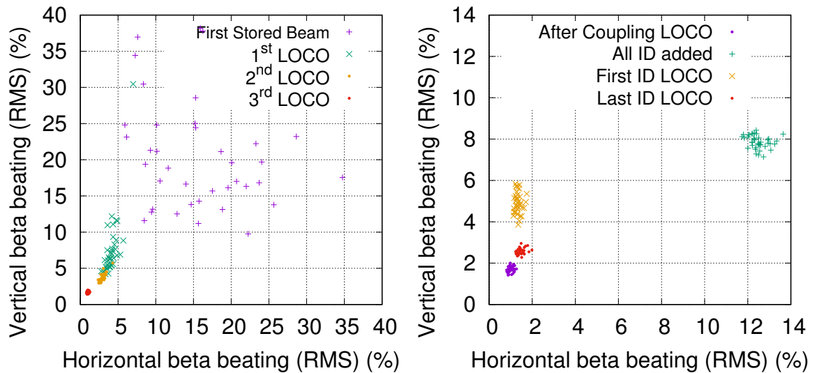
Figure 3. The distributions of the rms beta-beating at different stages. (Left: without ID. Right: with ID)
