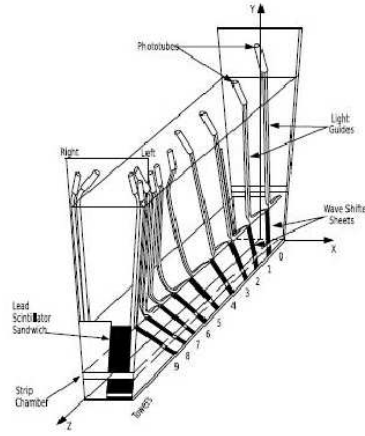
Figure 3.8: Light-shifter plates connected to light guides and to photomultipliers of the front electromagnetic compartment of a central calorimeter wedge.
