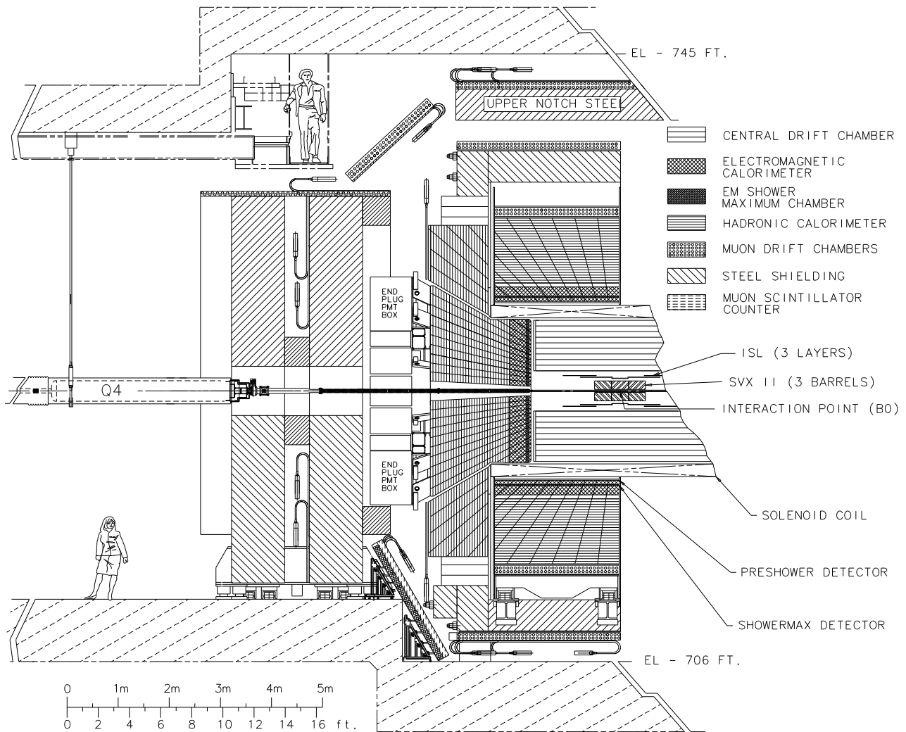
Figure 3.1: Elevation view of the CDF II detector
