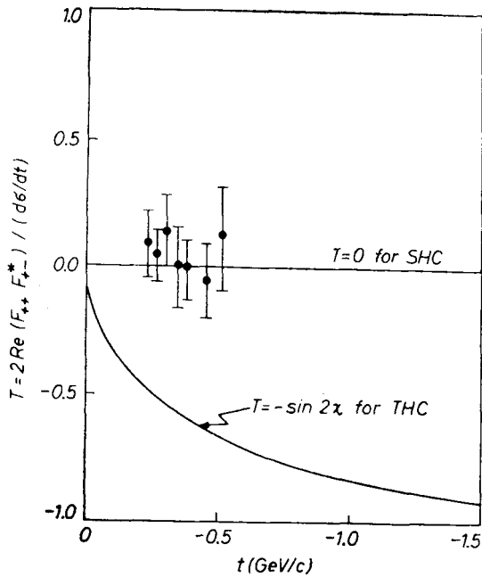
Fig. 1. The spin correlation parameter T (defined in the text) as a function of the four-momentum transfer t for \pi p \rightarrow \pi p at 6 GeV/c, together with the predictions for SHC ( T = 0 ) and THC ( T = -\sin 2\chi ) (taken from Ref. [6])
