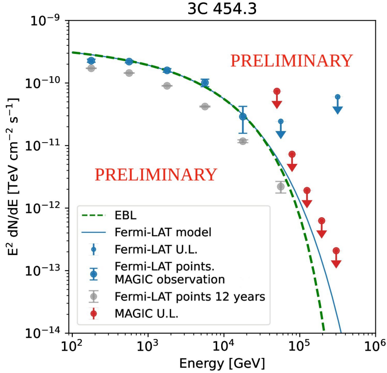
Figure 2: SED in GeV and VHE range for the source 3C 454.3: derived VHE differential upper limits (95 % C.L.) on the flux by MAGIC and Fermi -LAT spectrum obtained during the MAGIC observation period
