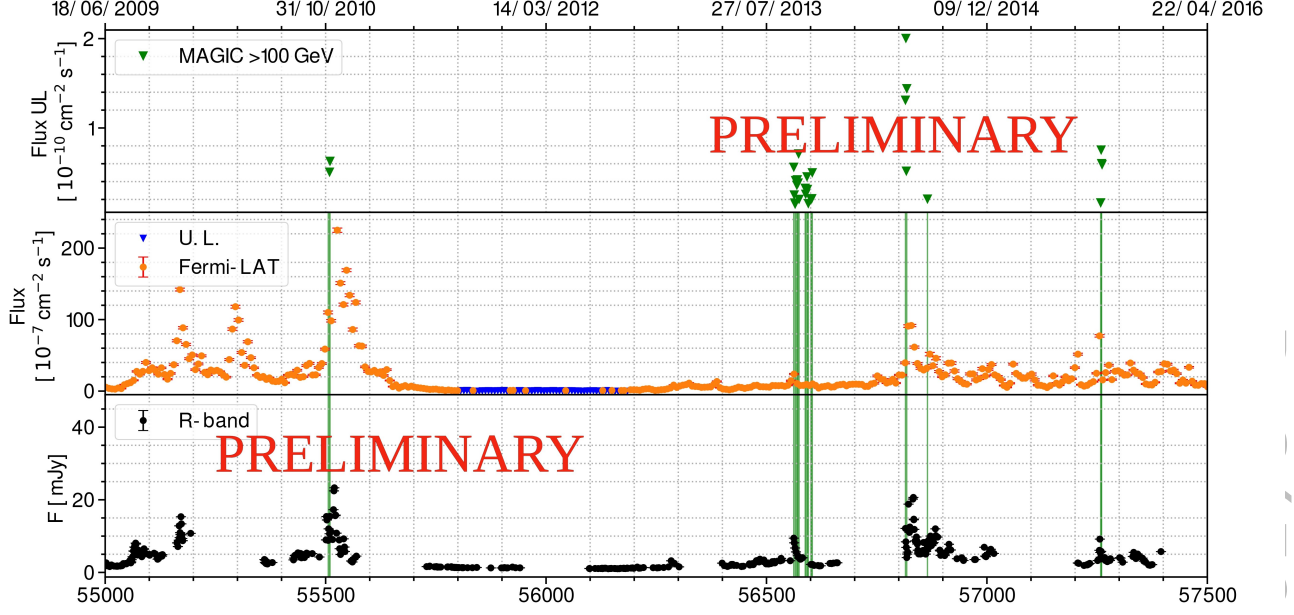
Figure 1: Light curve of 3C 454.3. The green vertical areas indicate the days during which MAGIC observations were carried out.
