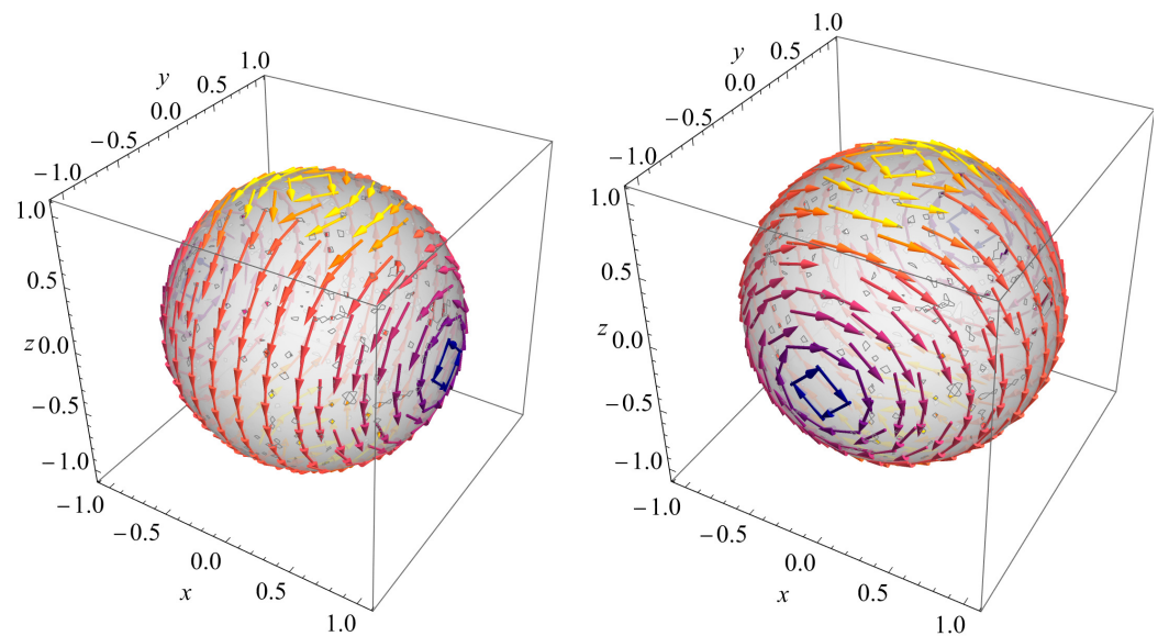
Figure 1. Sketches of the force lines of the components of the color current g\vec{j}^1 r^3 / (\hbar c uv) ( left panel ) and g\vec{j}^2 r^3 / (\hbar c uv) ( right panel ) on the surface r = \text{const} . The plots are given in Cartesian coordinates \{x, y, z\} .
