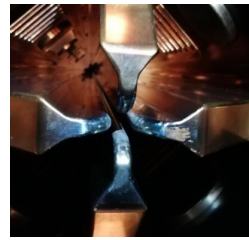
Figure 11: RFQ vane at the entrance before LEBT chopper rotation.
