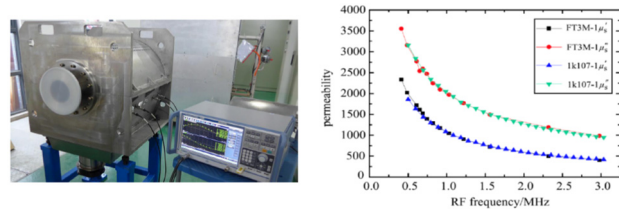
Figure 17 : Measurement(upper) of the domestically developed MA strip and its results(lower) in comparison with HITACHI products FT3M.
