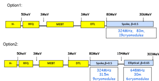
Figure 14 : Two options of the S.C. linac.
