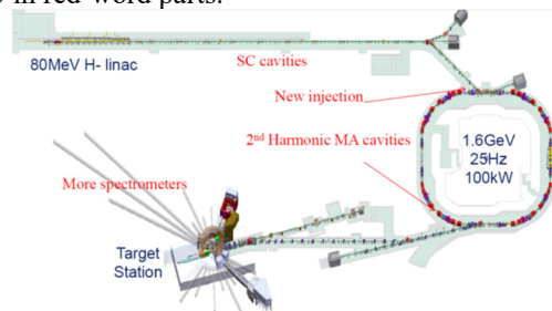
Figure 13: CSNS phase-2 major upgrade items (in red).
