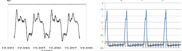
Figure 6: Bunching effect before(left) and after(right) RF optimization.
