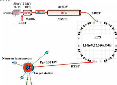
Figure 1: Schematics of the CSNS complex.
