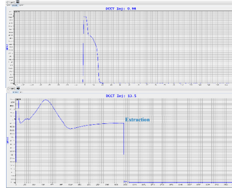
Figure 7: Beam current in RCS before(upper) and after (lower) timing tuning.
