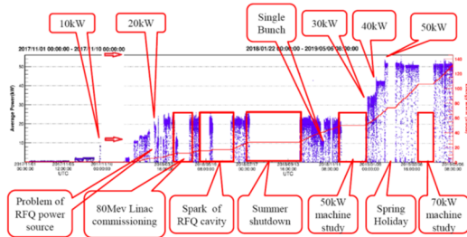
Figure 9: Overview of the beam power increase.
