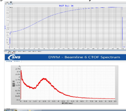
Figure 8: RCS beam transmission reached 100% (upper) and the first neutrons were generated on the target of CSNS(lower).
